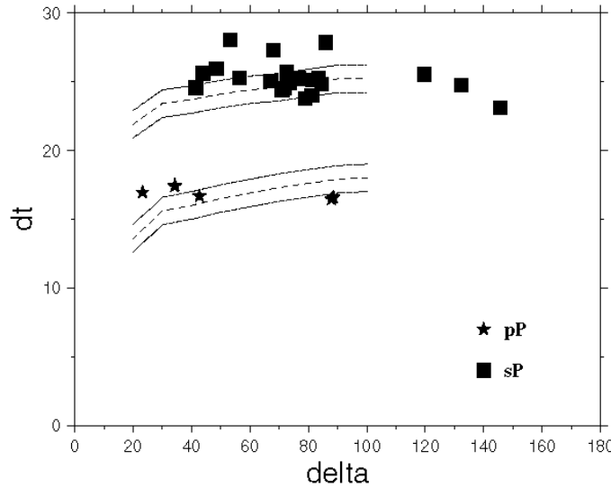
Figure 3: Travel time differences of pP-P (stars) and sP-P (squares) versus distance for a 04/01/98 REB event. The dashed lines represent the expected moveout, while the solid lines represent one-second deviations.
