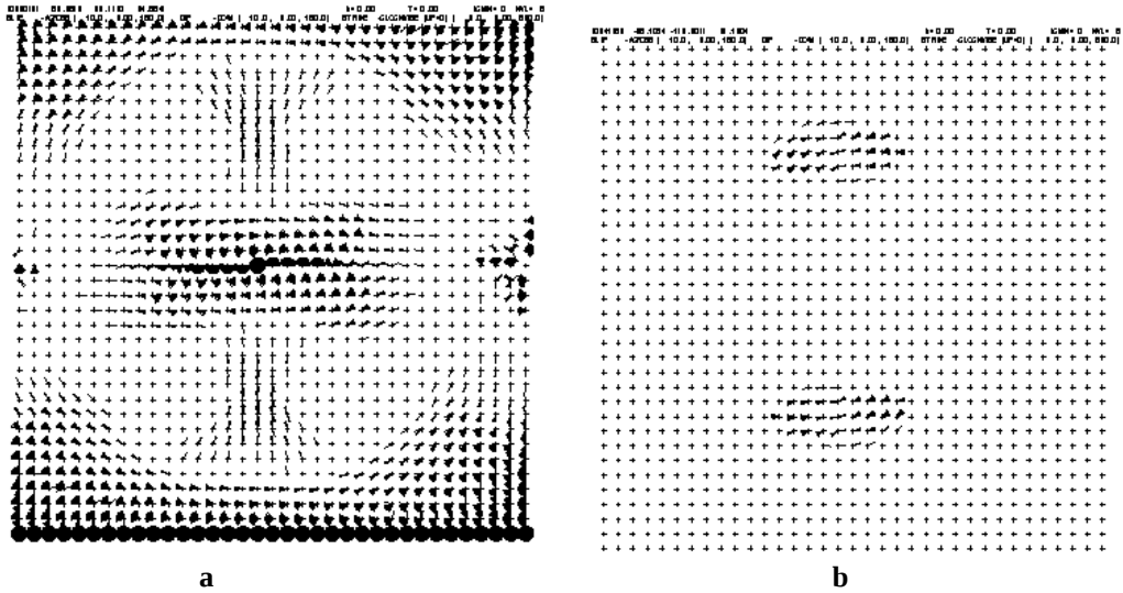
Figures 8 a & b: Double couple solutions consistent with the input data for the a) poorly constrained southern Greek event and the b) well-constrained Fijian event. The dip, slip are on the vertical and horizontal axes respectively, and the azimuth of the strike for consistent solutions is shown as a vector plotted at each dip-slip position.
