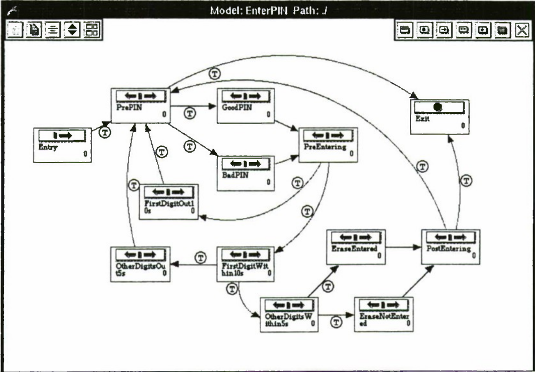
Figure 5 Finite State Machine Model for Enter PIN
