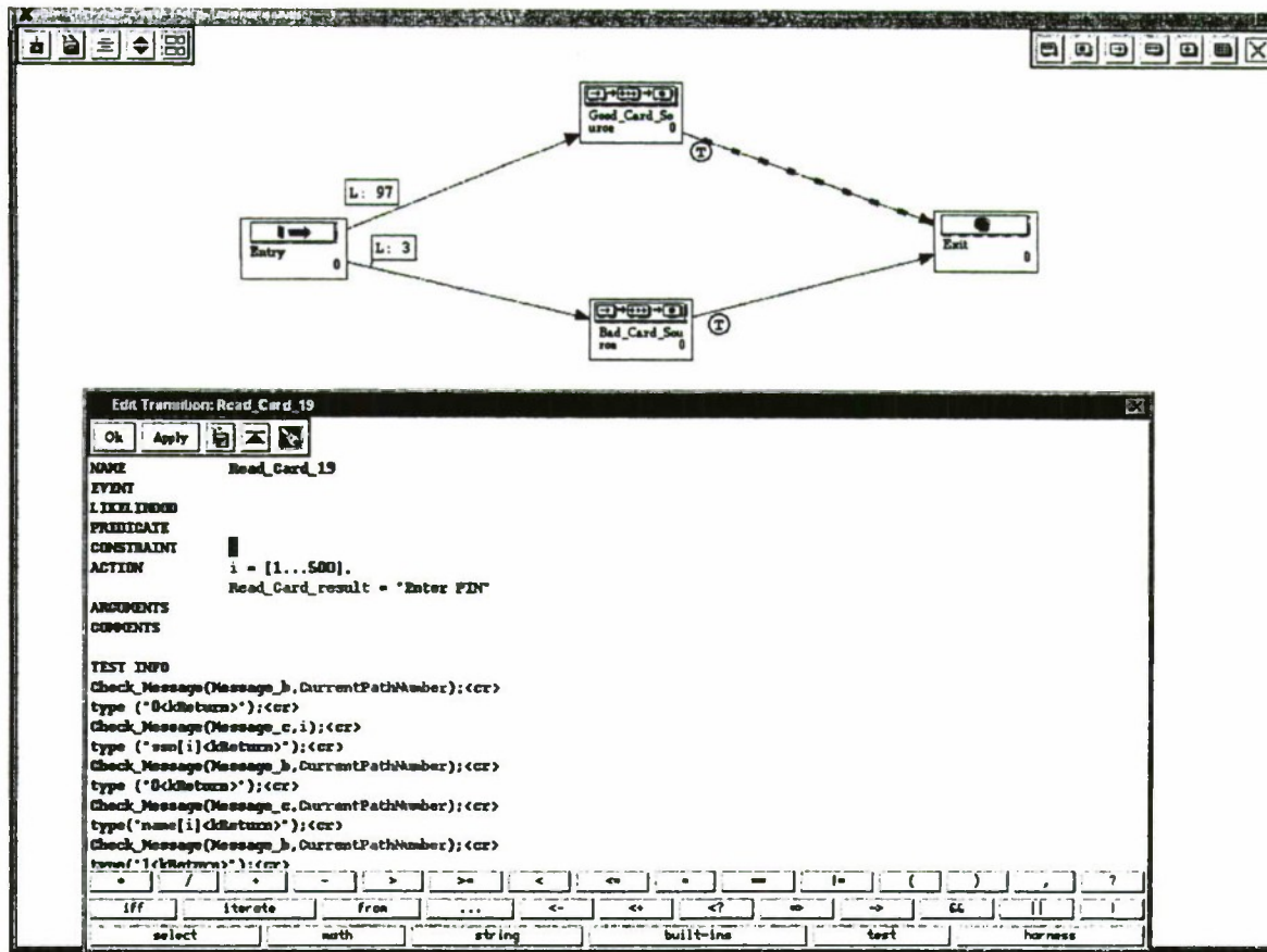
Figure 2 TestMaster Model Read_Card and Its Different Modeling Elements
