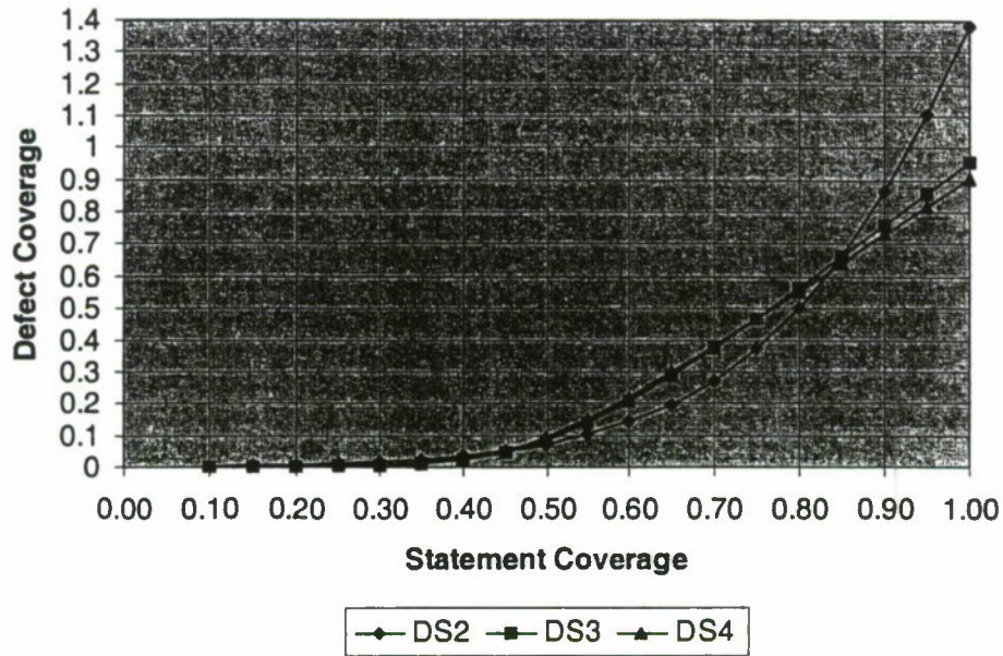
Figure 7 Fault Coverage vs. Test Coverage
