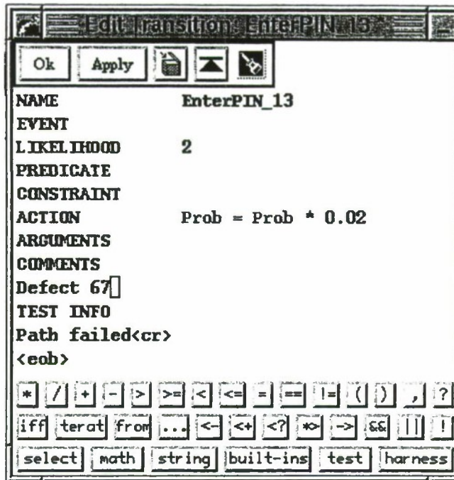
Figure 6 Parameters of the Transition Between the State PreEntering and FirstDigitOut10s
