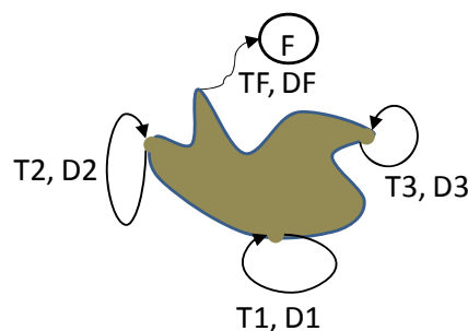
Figure 10. Lost-miner Problem
