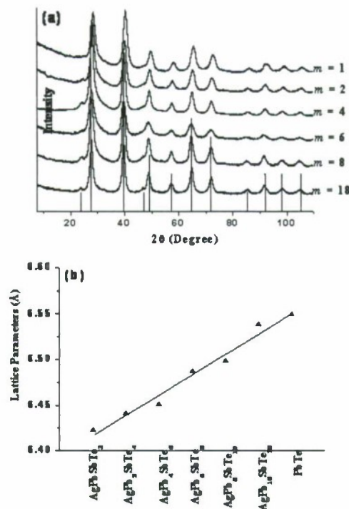
Figure 1. [a] Powder X-ray diffraction patterns of the \text{AgPb}_m\text{SbTe}_{m+2} ( m = 1-18 ) nanocrystals. The ICDD-PDF overlays of cubic PbTe (PDF # 08-0028) is shown as vertical lines. [b] A plot showing the change in lattice parameter (calculated based on the PXRD spectra) with the nominal atomic composition of \text{AgPb}_m\text{SbTe}_{m+2} nanocrystals.
