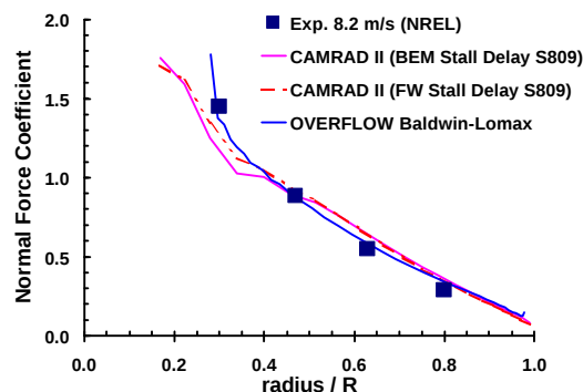
Figure 9: C_n vs. r/R Comparison between CAMRAD and OVERFLOW, 8.2 m/s average wind speed
