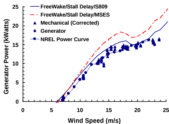
Figure 7: CAMRAD II power curve Experimental and computed airfoil tables
