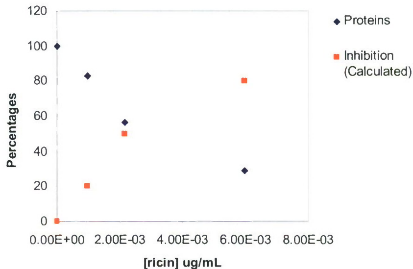
Figure 2. Calculated Percent Inhibition (orange squares) and Normalized Average Number of Proteins Identified (blue diamonds) Versus Ricin Dose
