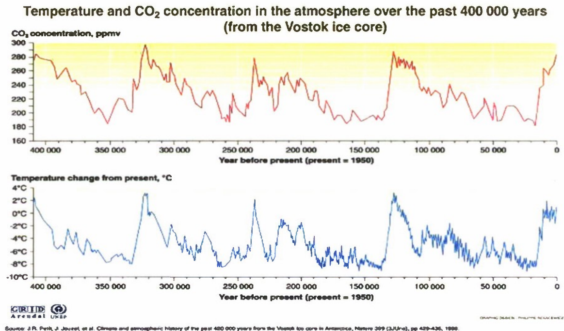
Figure 1. Relationship between Atmospheric CO 2 Levels and Temperature (Petit et al., 1999).
