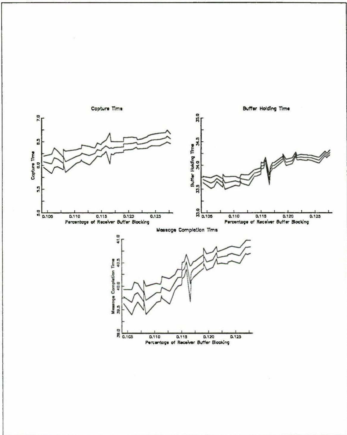
Figure 15. Influence of Total Number of Transmitted Messages on System Performance.
