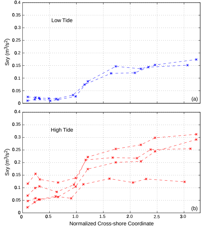
Figure 8. S_{xy}/\rho for the cases (October 10 and 11) shown in Figures 5 & 6 in the normalized cross-shore cross-shore coordinate x' (1). (a) low tide (b) high tide. The accuracy of S_{xy} estimates is limited because of uncertainties in current meter response and orientation, and because errors in linear theory may be significant in the surfzone. Only two low tide profiles are shown because of unavailable data.
