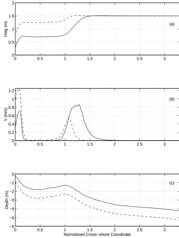
Figure 7. Modeled (a) significant wave heights (b) mean longshore currents (c) model bathymetry in normalized cross-shore coordinate (1). Solid curves represent low tide and dashed curves are high tide. The incident wave parameters are representative of conditions in Figure 5 and 6: H_{\text{sig}} = 1.5 m and \theta = 25^\circ .
