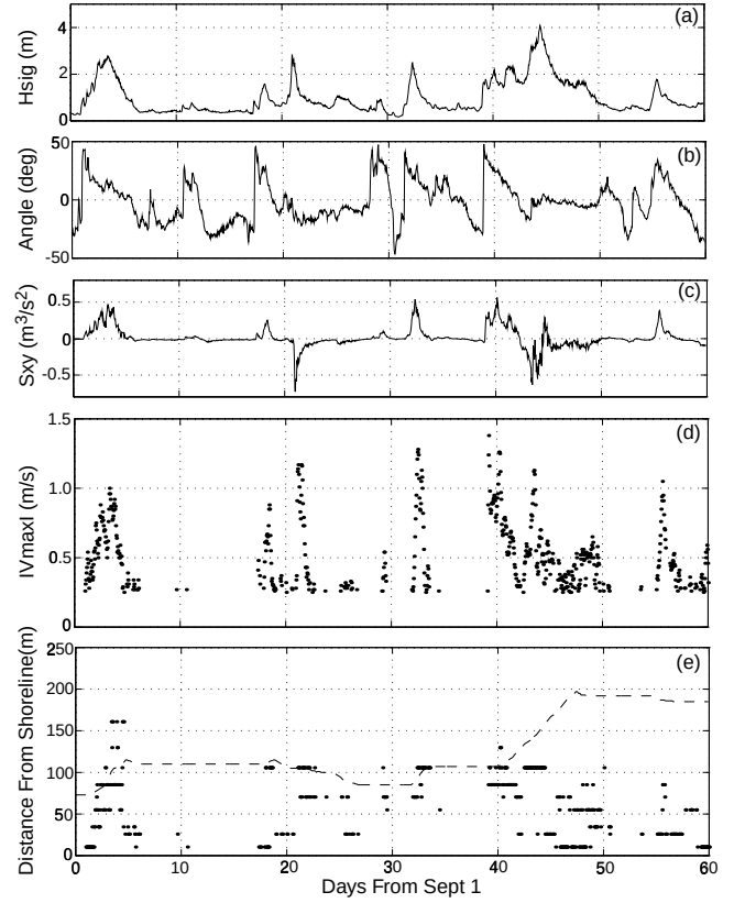
Figure 2. Hourly values of (a) significant wave height H_{\text{sig}} in 8 m depth (b) deviation of the mean incident wave angle from shore normal (positive angles correspond to waves from the northern quadrant) (c) S_{xy}/\rho in 8 m depth (d) maximum hour-averaged longshore current \bar{v}_{\max} (e) bar crest location (dashed) and the cross-shore location \bar{v}_{\max} . \bar{v}_{\max} is plotted only if there were at least five active current meters and \bar{v}_{\max} \geq 0.25 m/s. Out of 1464 possible values, 572 hourly maxima pass these criteria. The few maxima occurring more than 250 m from shore are not shown in (e).
