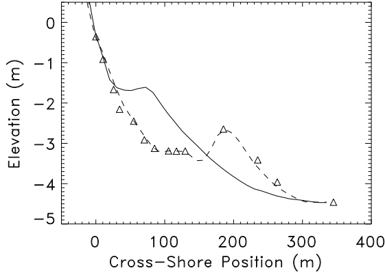
Figure 1. The cross-shore location of current meters ( \Delta ), and measured bathymetry relative to sea level on August 25 (solid line) and October 26 (dashed line). An additional current meter located at cross-shore location 749 m in 8 m water depth is not shown.
