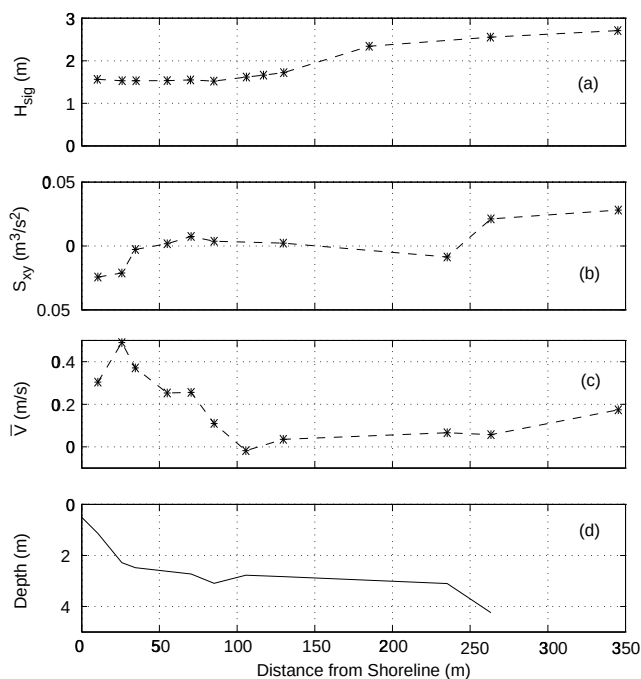
Figure 9. Observed cross-shore variation of (a) significant wave height (b) S_{xy}/\rho (c) longshore current \bar{v} (d) bathymetry on 0500 October 10.
