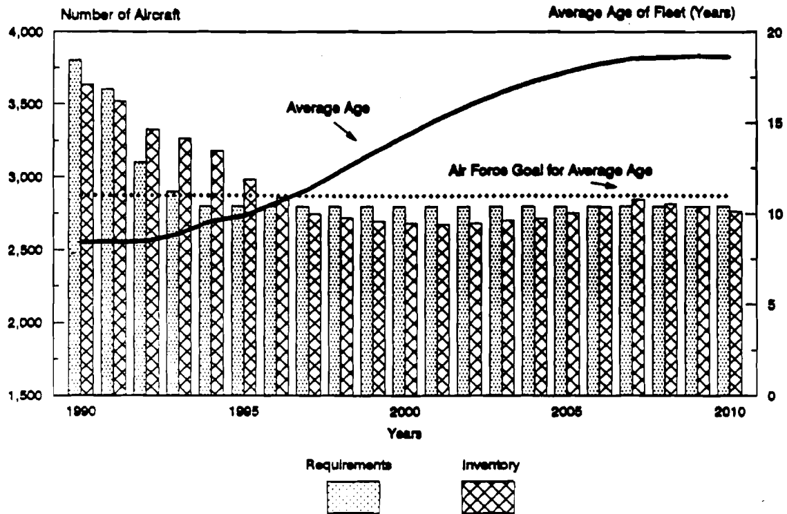
FIGURE 2. AIR FORCE INVENTORY, REQUIREMENTS, AND AVERAGE AGE (Assumes Aircraft Are Retained to Meet Requirements – About 28 Years)
