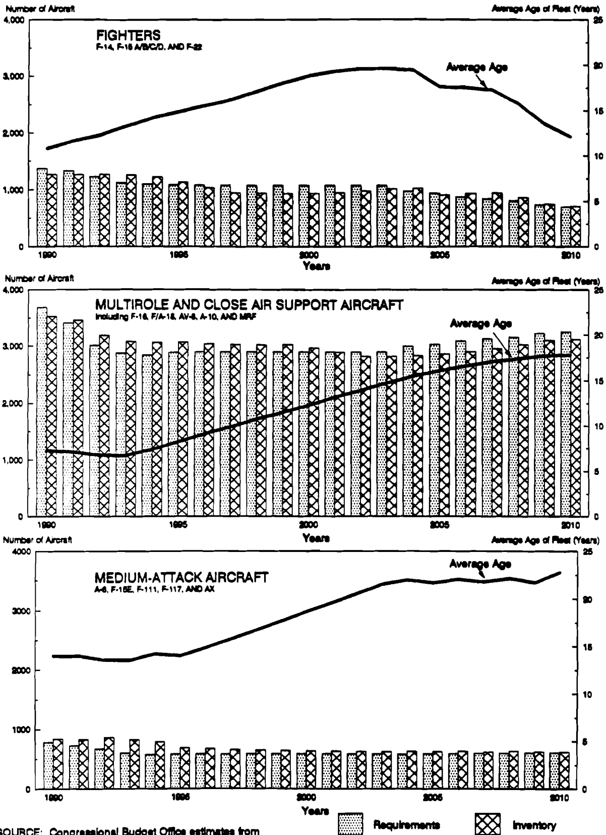
FIGURE 7. INVENTORY, REQUIREMENTS, AND AVERAGE AGE OF AIRCRAFT BY MISSION CATEGORY
