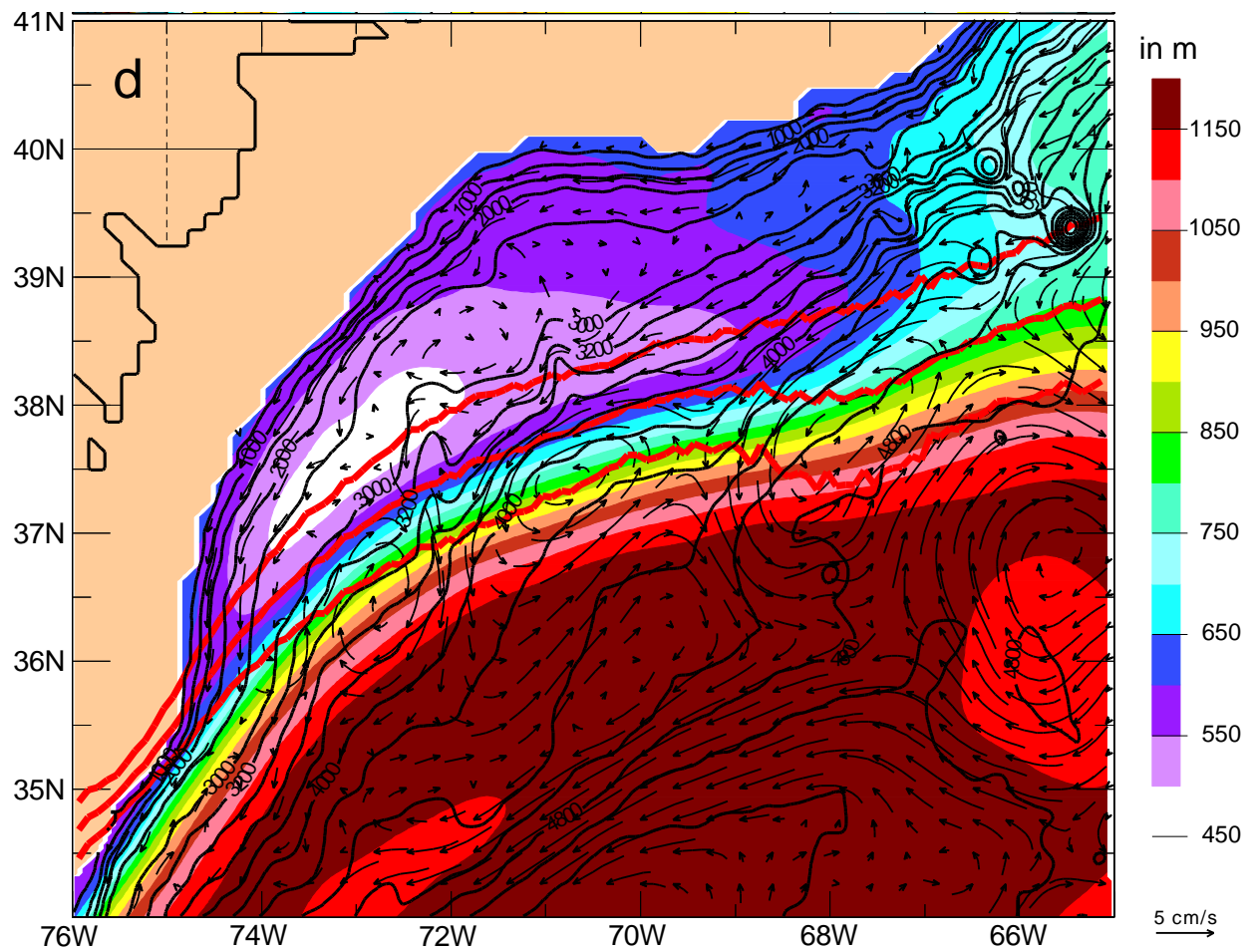
Fig. 7. Same as Fig. 4a but with isotachs (in color) replaced by the mean depth at the base of the model thermocline (in color), i.e. the mean depth of the interface between layer 4 and layer 5 (the abyssal layer) from the 1/32^\circ simulation depicted in Figs. 2c and 3c. [From Hurlburt and Hogan, 2008]
