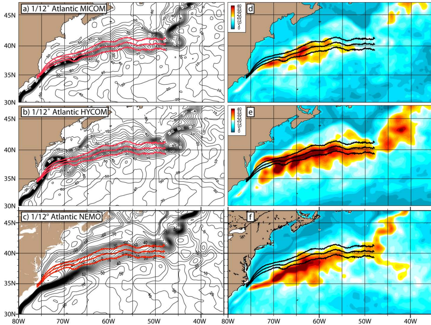
Fig. 10. Mean SSH (left column) and mean SSH variability (right column) from (a,d) a 1/12° Atlantic MICOM simulation over 1982-1983, (b,e) a 1/12° Atlantic HYCOM simulation over years 11-13, and (c,f) a 1/12° Atlantic NEMO simulation over 2004-2006. The contour interval in both columns is 5 cm. The mean Gulf Stream IR northwall pathway \pm 1\sigma from Cornillon and Sirkes is overlaid on each panel in red in the left column and black in the right column.
