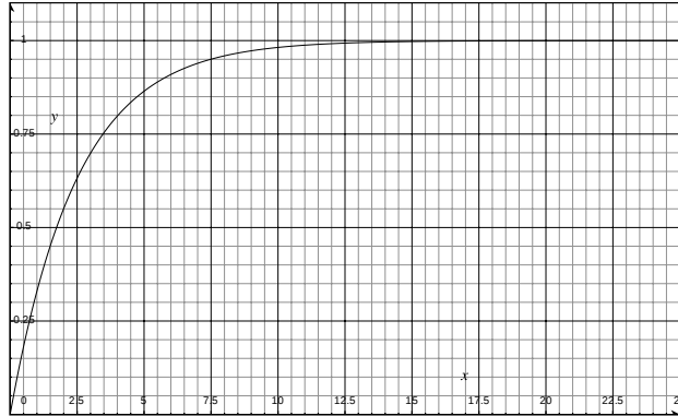
Figure 4: U(x) = 1 - e^{-x \cdot 0.4}
