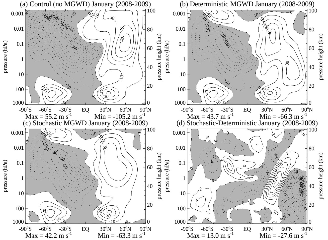
FIG. 8. Zonal-mean zonal winds ( \text{m s}^{-1} ) for January 2008-2009 from NOGAPS-ALPHA nature runs: (a) control run without nonorographic gravity wave drag, and runs using the (b) deterministic and (c) stochastic parameterizations of nonorographic gravity wave drag with equivalent settings to produce the same time-mean drag. Differences in the zonal-mean zonal winds between the stochastic and deterministic simulations are plotted in (d).
