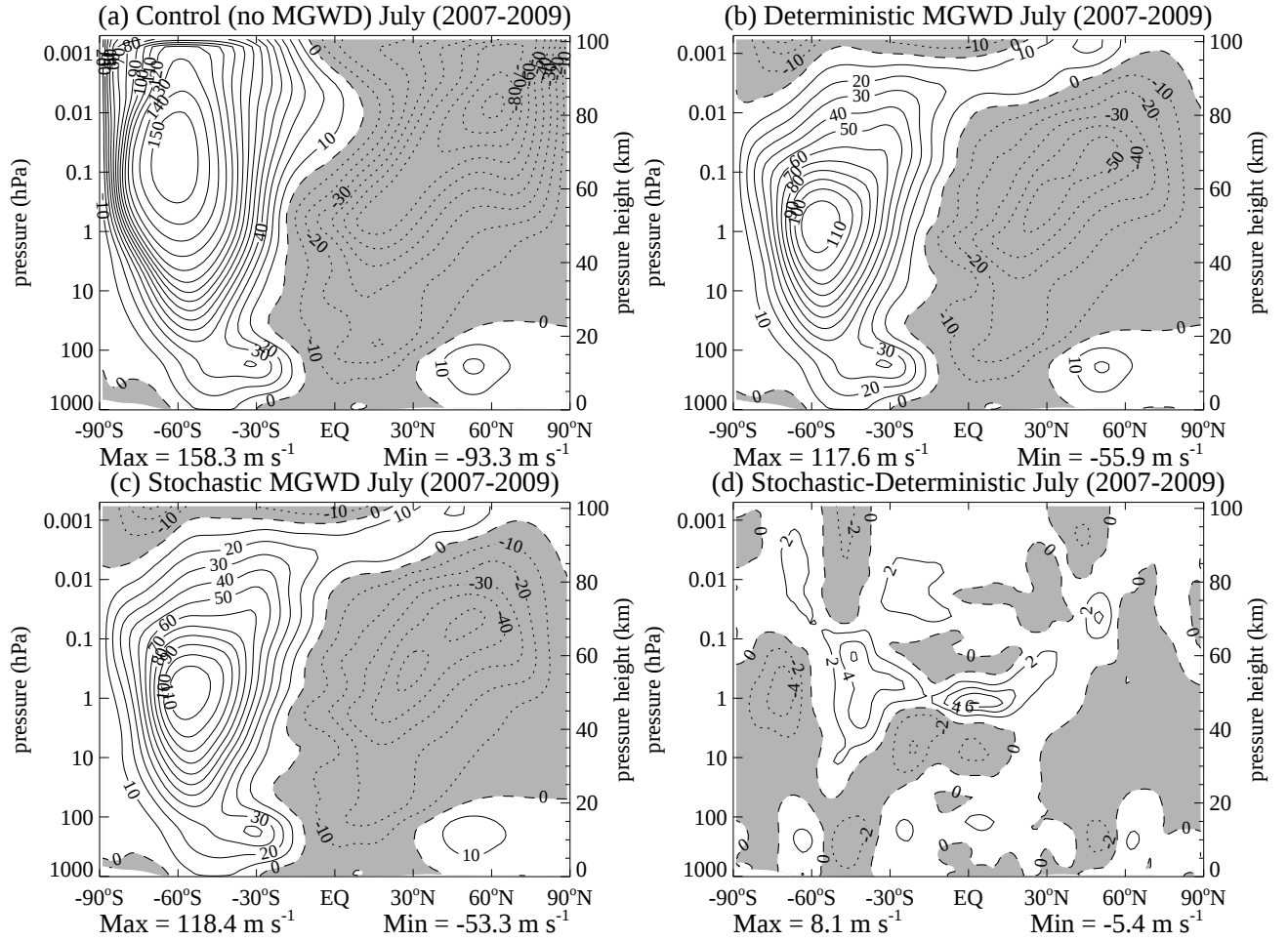
FIG. 6. Zonal-mean zonal winds ( \text{m s}^{-1} ) for July 2007-2009 from NOGAPS-ALPHA nature runs: (a) control run without nonorographic gravity wave drag, and runs using the (b) deterministic and (c) stochastic parameterizations of nonorographic gravity wave drag with equivalent settings to produce the same time-mean drag. Differences in the zonal-mean zonal winds between the stochastic and deterministic simulations are plotted in (d).
