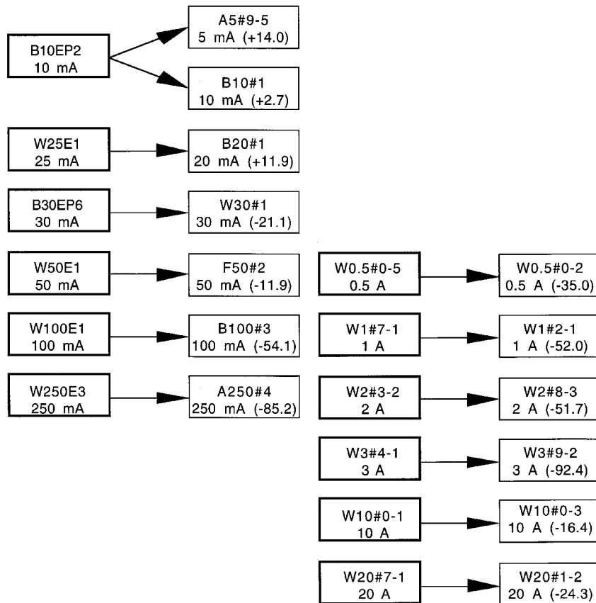
Fig. 4. Crossover or direct comparison between the reference standards and the working standards at rated current, in \mu A/A .
