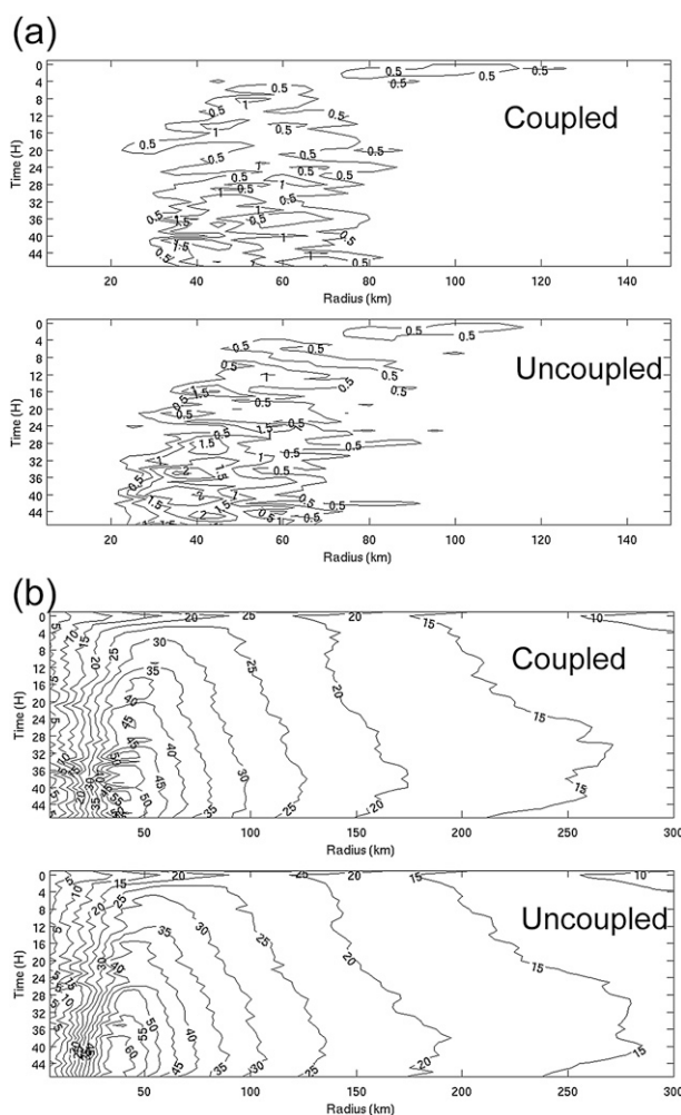
FIG. 11. Hovmöller diagram of azimuthally averaged (a) vertical velocity ( \text{m s}^{-1} ) at 700 hPa and (b) tangential wind ( \text{m s}^{-1} ) at 10 m. The contour interval is 0.5 \text{ m s}^{-1} for the vertical velocity and 5 \text{ m s}^{-1} for the tangential wind.
