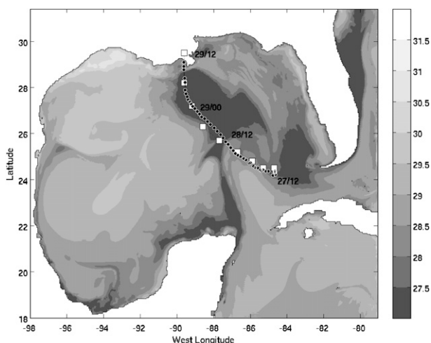
FIG. 5. Model-simulated SST ( ^\circ\text{C} ) at 48 h from ocean grid 1. The white squares denote the observed location of the eye at 6-h intervals and the dotted line denotes the model location of the eye at hourly intervals beginning at 1200 UTC 27 Aug 2005.
