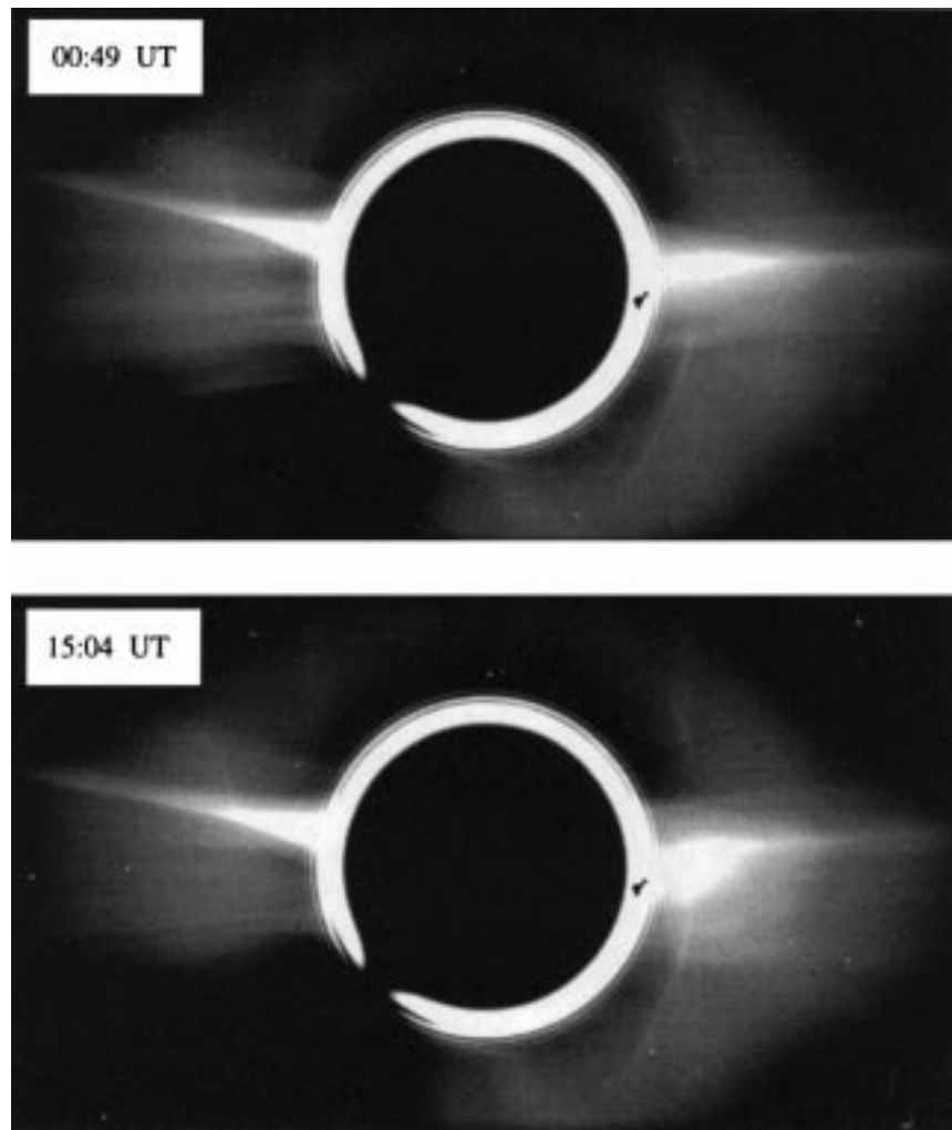
Figure 2. The growth of the streamer on July 28. The images are from the C2 coronagraph, where the diameter of the occulting disc is 1.5 R_{\odot} . The times of the images are in the upper left of each frame. The west limb is to the right and north is at the top on all figures. The image is taken with a clear filter and polarizer. The appearance of the west equatorial streamer at 00:49 UT was similar to that over the previous 12 hours. The image at 15:04 UT shows not only a significant brightening, but also a marked swelling. Note that the appearance of the east limb is little changed.
