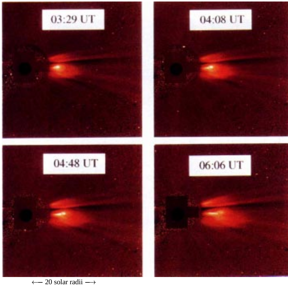
Figure 4. The ejection as seen in the C3 coronagraph, in four images taken at 03:29, 04:08, 04:48, and 06:06 UT, respectively. These images have all had a pre-event image subtracted, and therefore may contain some artefacts caused by rotation of the streamer. The appearance of the transient bright feature is not affected by this. This sequence shows the evolution of the height of the ejected mass with the bright, thin column linking back to the Sun.
