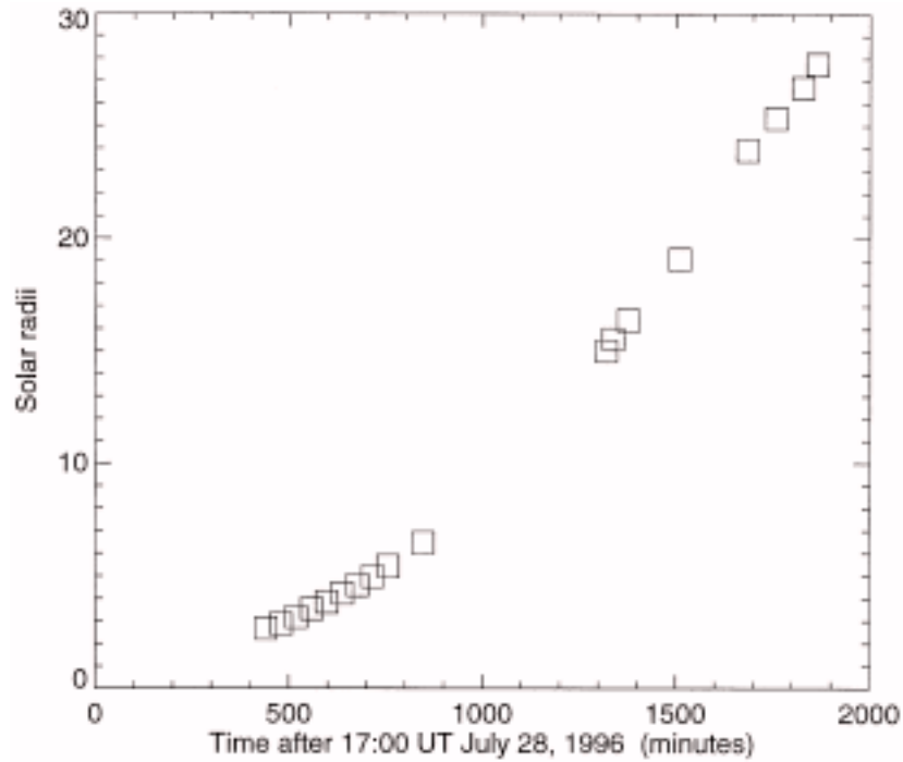
Figure 6. The height–time plot of the apex of the ‘<’, clearly identified in Figure 5. The velocity in the lower part of the plot is 110 \pm 5 \text{ km s}^{-1} and in the outer region it is 269 \pm 10 \text{ km s}^{-1} .
