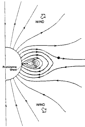
Figure 1. A model of the magnetic topology in a helmet streamer overlying a prominence. The lines of force in the high equatorial region enclose the equatorial interplanetary current sheet. Regions of high density are shaded. The closed magnetic field in the low-density cavity is normally in static equilibrium. The vertical prominence sheet is shown as a line extending out into the low density cavity. In this model the length runs in the azimuthal direction. (After Low, 1994.)
