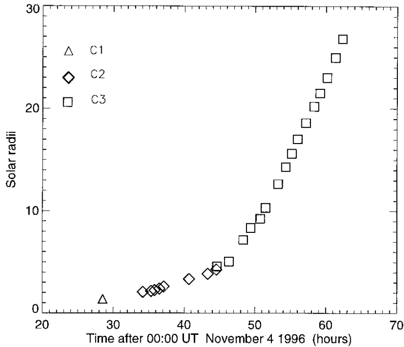
Figure 10. The height-time profile of the trailing edge of the mass ejection for the November 5 event. The different symbols indicate the coronagraph which has imaged the event at the indicated times.
