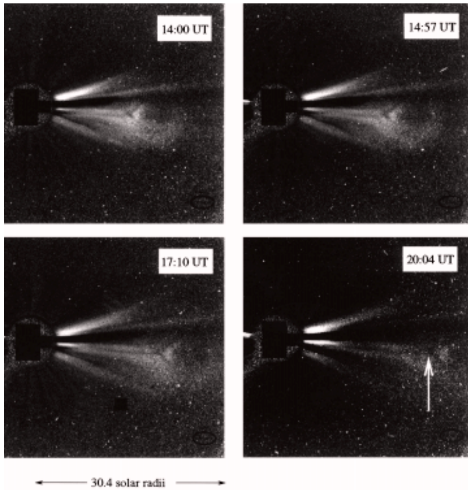
Figure 5. The motion of a '<' shaped rarefaction which developed behind the ejected mass. It is visible in the centre of the image taken at 14:00 UT on July 29. By 17:10 UT it is still quite clear, but by 20:04 it is becoming difficult to identify. The white arrow points to the apex of the '<' in this last frame. The projected angle, in the plane of the sky, between the two dark lines in the '<' is 75^\circ .
