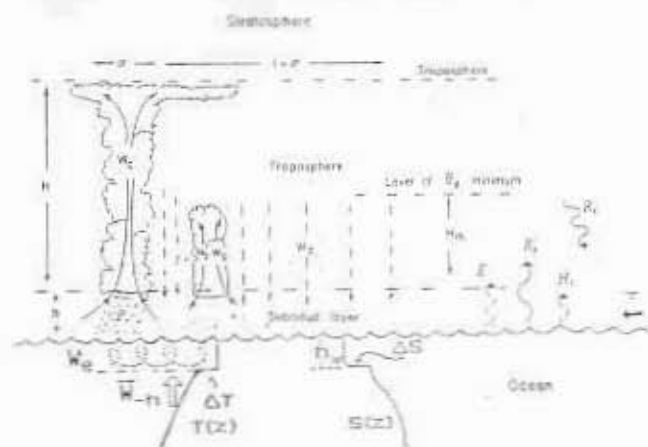
Fig. 2. Schematic presentation of the AOSHE model.
