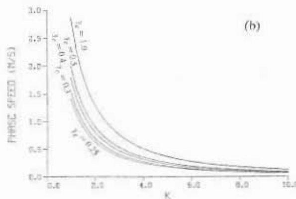
Fig. 3. Dependence of the AOSHE mode (under strong wind forcing) on the parameter \gamma_e : (a) growth rate ( \text{yr}^{-1} ), and (b) phase speed ( \text{m s}^{-1} ) for \gamma = 0.02 .
