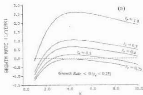
Fig. 1. Atmospheric convection generated by air-ocean feedback under (a) weak wind forcing, and (b) the strong wind forcing.
