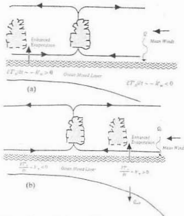
Fig. 1. Atmospheric convection generated by air-ocean feedback under (a) weak wind forcing, and (b) the strong wind forcing.
