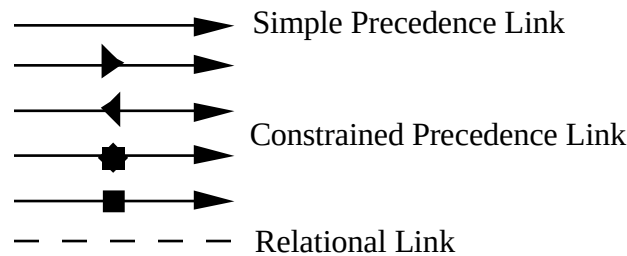
Figure 3-2 IDEF3 Link Types
