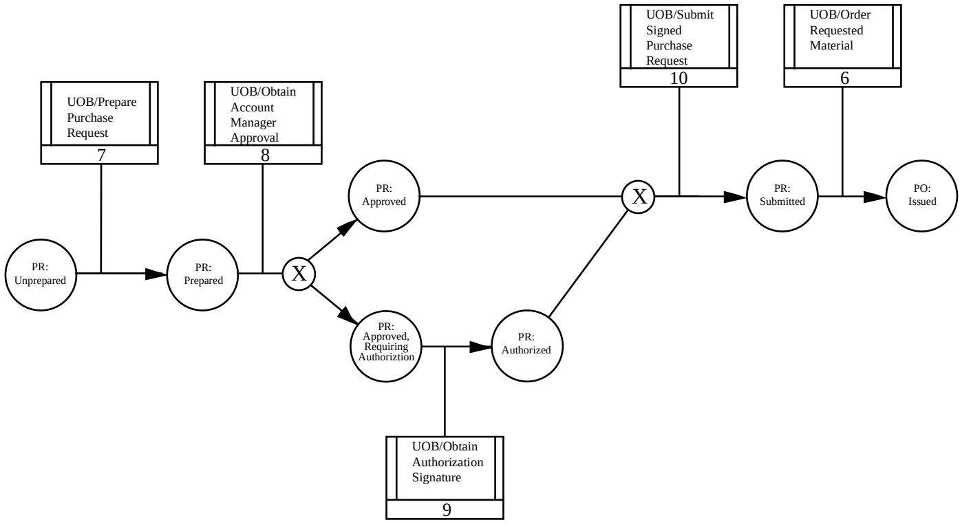
Figure 5-17 Complete Schematic Before First Review
