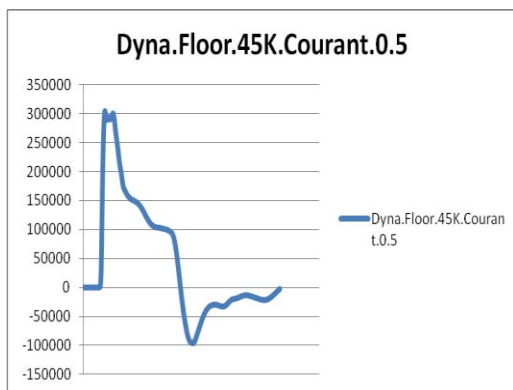
Floor Force by LS-Dyna (Newton) Figure (11)
