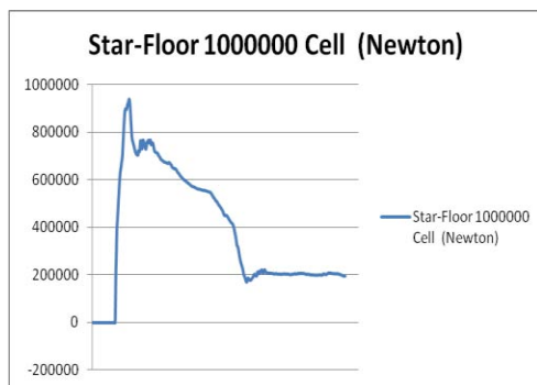
StarCCM+ Floor force 1,000,000 Mesh Density Figure (26)
