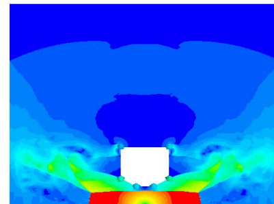
Mach No. StarCCM+ Figure (9)
