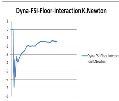
LS-Dyna FSI Floor Interaction Force Figure (34)
