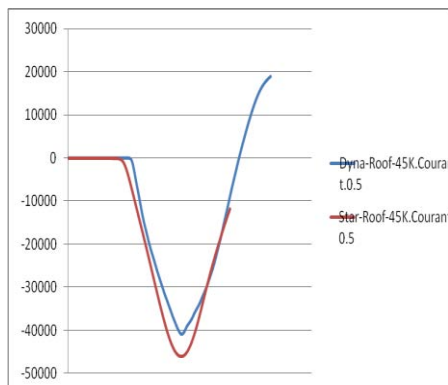
Roof Force (N) StarCCM+ & LS-Dyna StarCCM+ supersonic pressure = 1.0 bar Figure (21)
