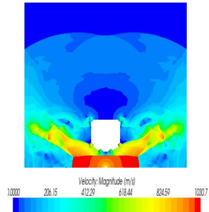
Velocity Distribution StarCCM+ Figure (8)
