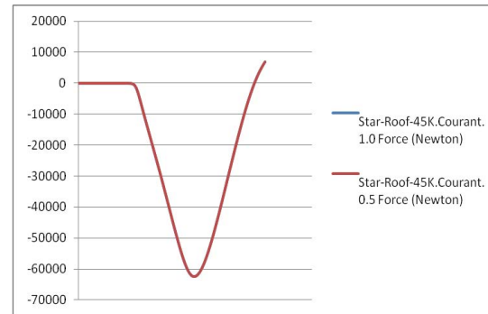
Total Roof Force comparison StarCCM+ variation Courant setting 0.5-1.0 (Note: lines are the same) Figure (19)
