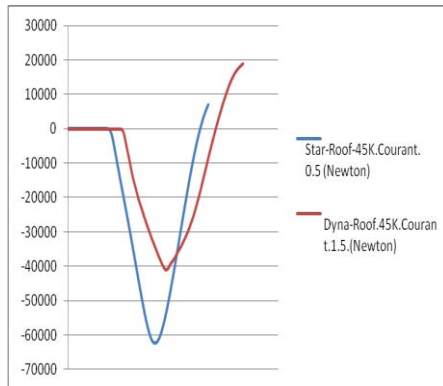
Roof Force StarCCM+ & LS-Dyna Figure (14)
