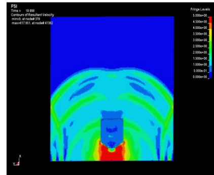
LS-Dyna FSI Pressure fluctuations Figure (31)
