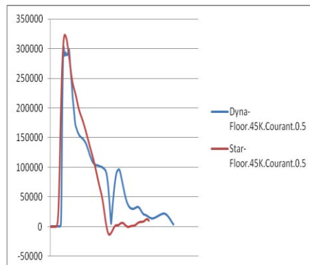
Floor Force (N) StarCCM+ & LS-Dyna StarCCM+ supersonic pressure = 1.0 bar Figure (20)
