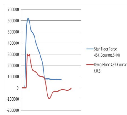
Floor Force StarCCM+ & LS-Dyna Figure (13)
