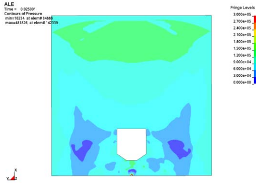
LS-Dyna Pressure fluctuations Figure (29)
