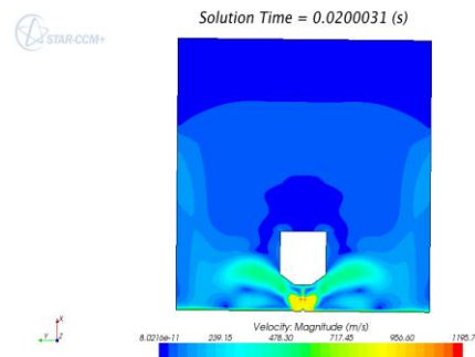
Star-CCM+ Velocity fluctuations Figure 23
