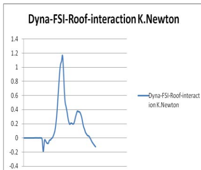
LS-Dyna FSI Roof Interaction Force Figure (35)
