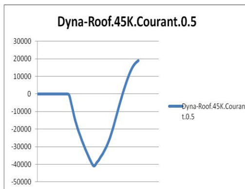
Roof Force by LS-Dyna (Newton) Figure (12)
