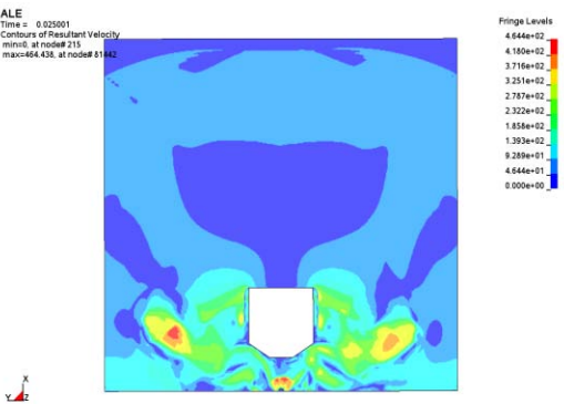
LS-Dyna Velocity fluctuations Figure (30)
