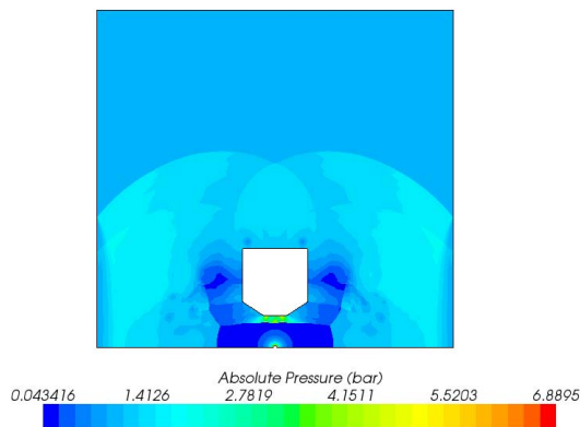
Pressure Distribution StarCCM+ Figure (7)
