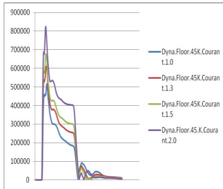
Total Floor Force (N) comparison LS-Dyna variation Courant setting 1.0-2.0 Figure (17)
