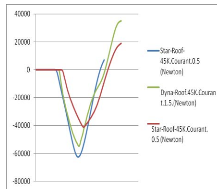
Roof Force StarCCM+ & LS-Dyna Courant 0.5-1.0 Figure (16)
