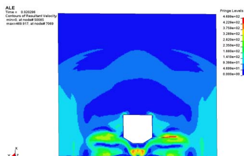
LS-Dyna Velocity fluctuations Figure 22
