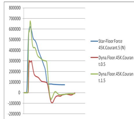
Floor Force StarCCM+ & LS-Dyna Courant setting 0.5-1.0 Figure (15)
