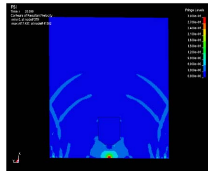
LS-Dyna FSI Pressure fluctuations Figure (32)
