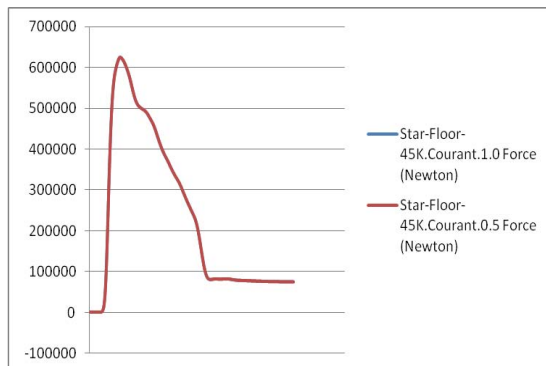
Total Floor Force comparison StarCCM+ variation Courant setting 0.5-1.0
