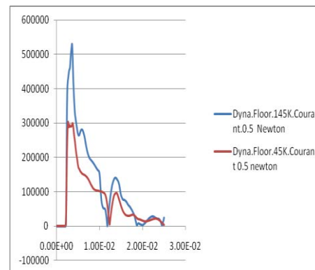
LS-Dyna 45K and 145K Mesh Density Floor Force (N) Comparison for Courant-0.5 Figure (28)
