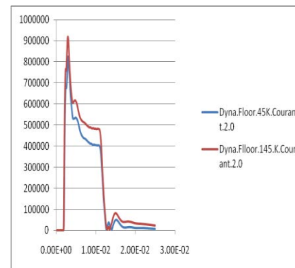
LS-Dyna 45K and 145K Mesh Density Floor Force (N) Comparison for Courant-2.0 Figure (27)
