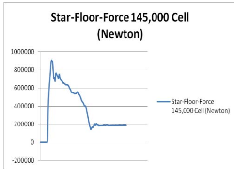
StarCCM+ Floor force 145,000 Mesh Density Figure (25)
