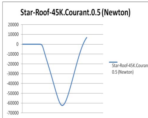
Roof Force by StarCCM+ Figure (6)
