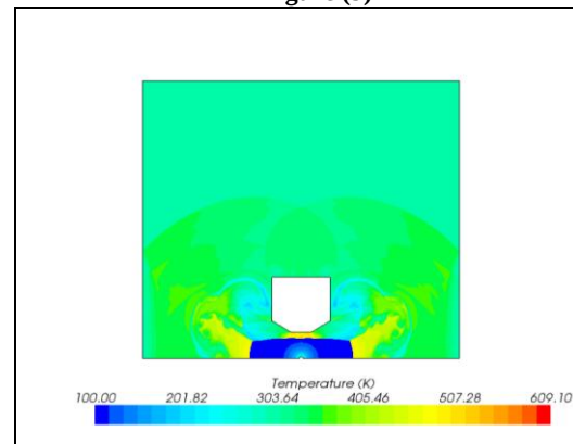
Temperature Distribution StarCCM+ Figure (10)
