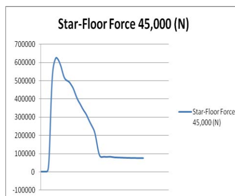
Floor Force by StarCCM+ Figure (5)
