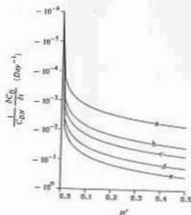
Fig.5. Dependence of 1/C_{DN} \partial C_D / \partial t on the cloudiness disturbance n' for \gamma = 5.0 (ocean gaining heat), and for: (a) \xi = 0.01 \text{ m/day} , (b) \xi = 0.05 \text{ m/day} , (c) \xi = 0.1 \text{ m/day} , (d) 0.25 \text{ m/day} , and (e) 0.5 \text{ m/day} .
