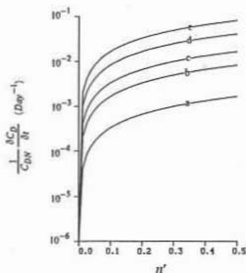
Fig.4. Dependence of 1/C_{DN} \partial C_D / \partial t on the cloudiness disturbance n' for \gamma = 0.1 (ocean losing heat), and for: (a) \xi = 0.01 \text{ m/day} , (b) \xi = 0.05 \text{ m/day} , (c) \xi = 0.1 \text{ m/day} , (d) 0.25 \text{ m/day} , and (e) 0.5 \text{ m/day} .
