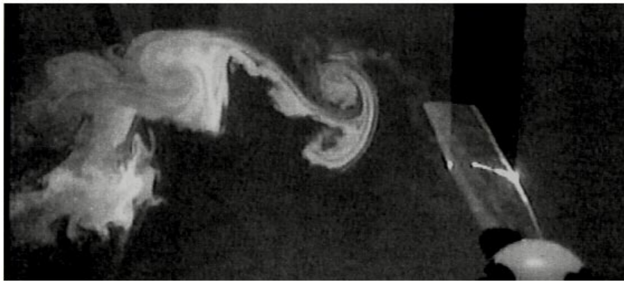
Figure 8. Laser Light Sheet Flow Visualization of Trailed Tip Vortices
