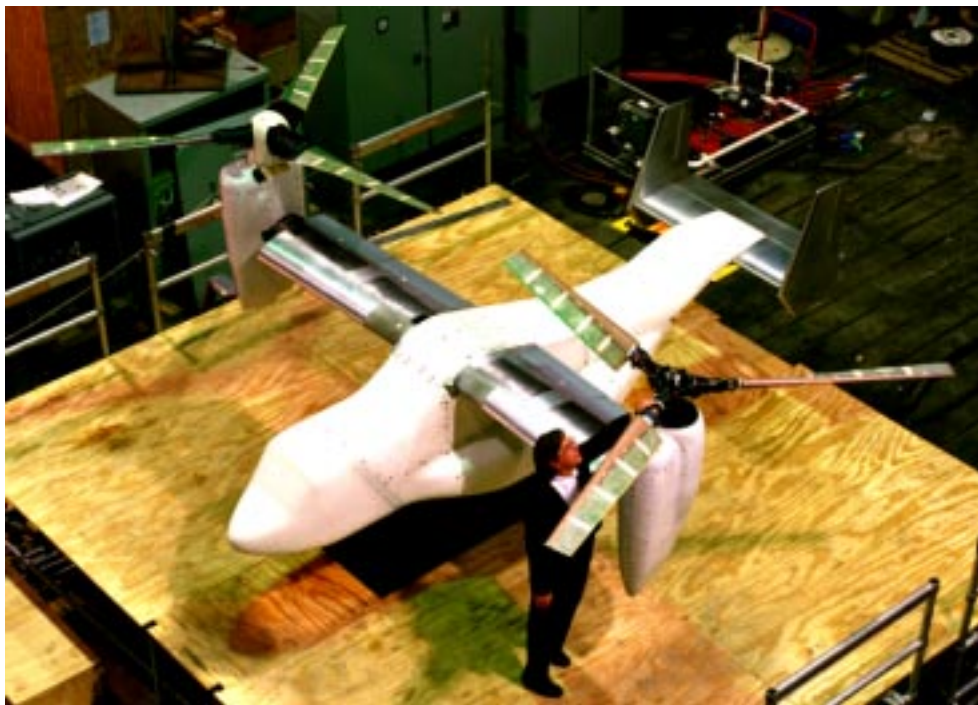
Figure 3. Full-span TRAM configuration
