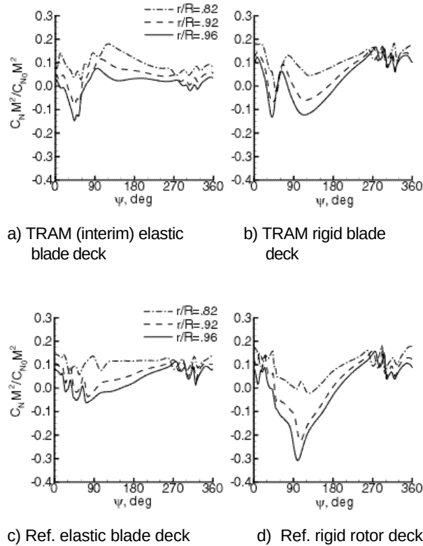
Figure 7. Predicted local blade normal force (normalized) determined using the rigid and elastic blade motion modeling in the TRAM Reference model decks (TRAM rotor condition of low C_T , \alpha_s = 6^\circ , \mu = 0.175 ).
