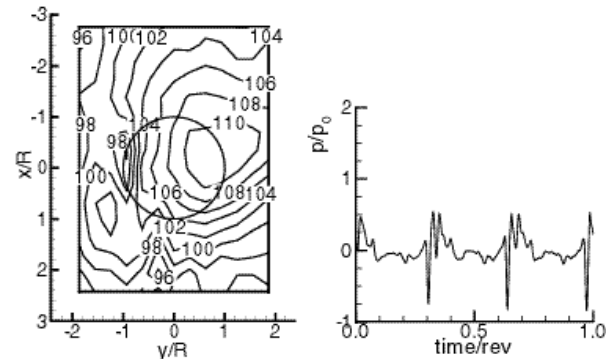
Figure 10. Measured TRAM BVISPL (dB-dB 0 ) contour and measured time history obtained from location-A under the advancing side (Figure 9). (TRAM rotor condition of low C_T , \alpha_s = 6^\circ , \mu = 0.175 ).
