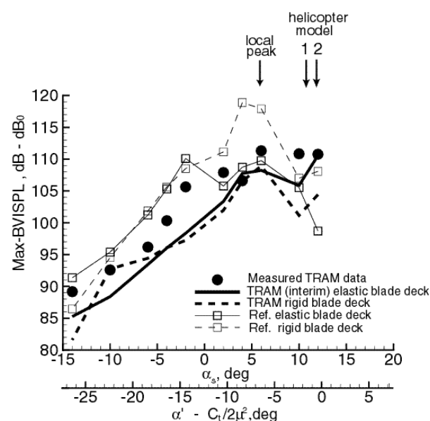
Figure 13. Max-BVISPL on advancing side for low C_T condition, \mu=0.15 .
