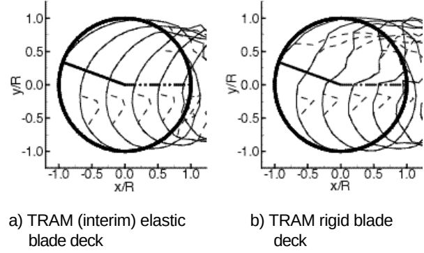
Figure 8. Top view of predicted wake geometry for the TRAM rotor. (Rotor condition of low C_T , \alpha_s = 6^\circ , \mu = 0.175 ).
