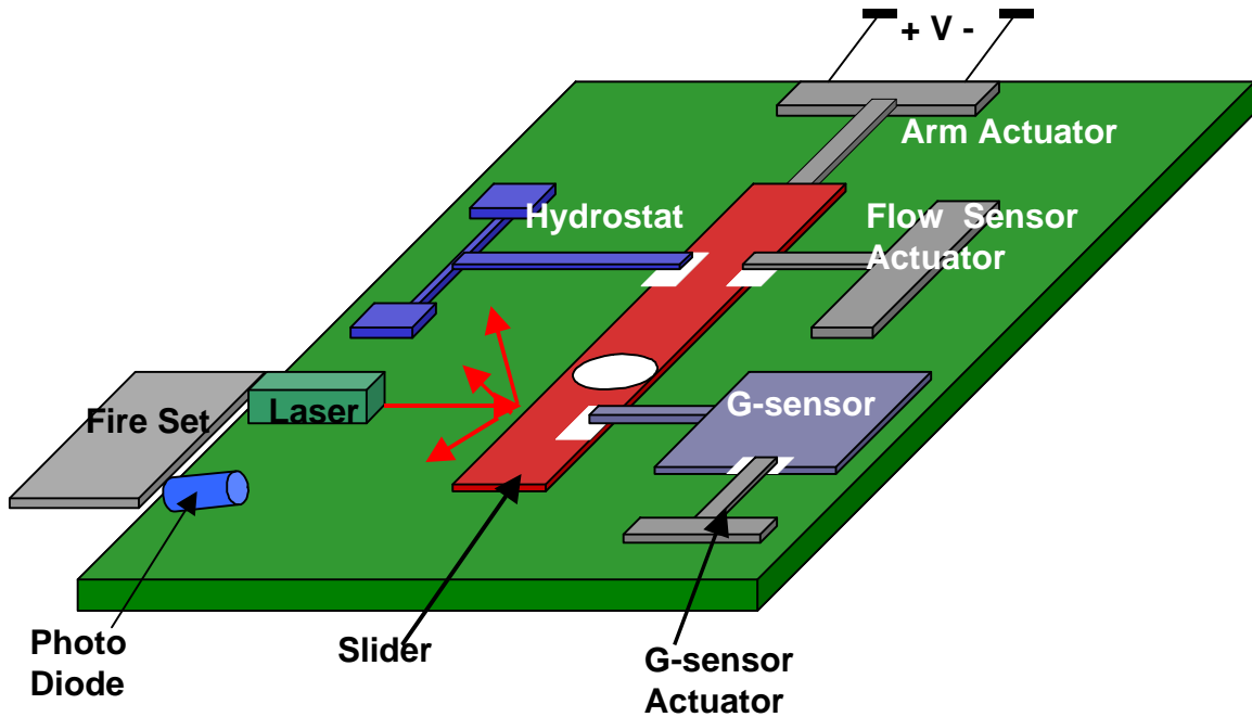
Fig. 4. Key components of the S&A fuze systems.
