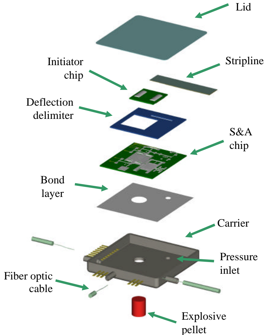
Fig. 5 Carrier-level package.
