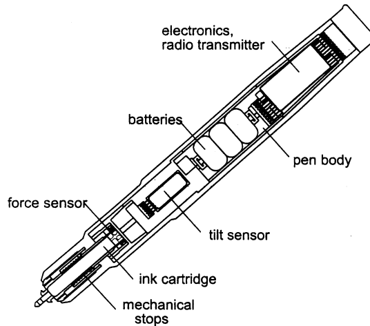
Fig. 1. SmartPen system [1] (Courtesy of IEEE).
