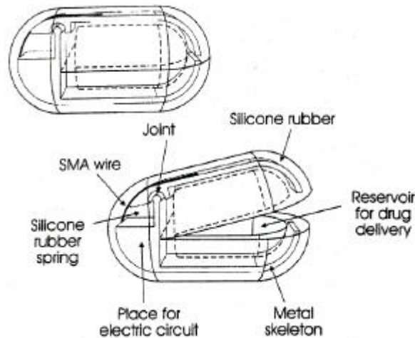
Fig. 2. Solid drug delivery device [1] (Courtesy of IEEE).
