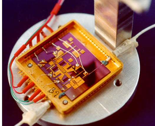
MEMS Safety & Arming Chip
