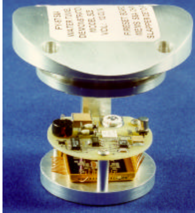
Torpedo Safety & Arming/Fuzing Prototype System
