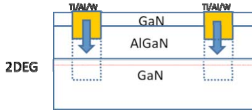
Figure 8: Schematic cross section of the fabricated GaN/AlGaN/GaN with recess.
