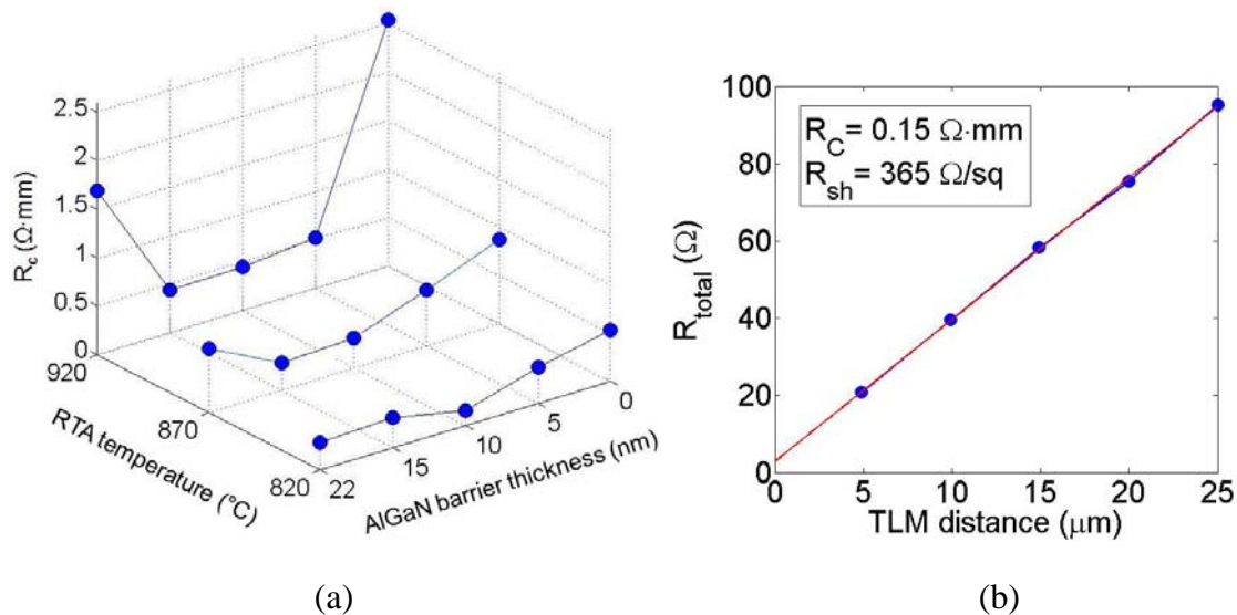
Figure 10. (a) Measured contact resistance ( R_c ) as function of RTA temperature and remaining AlGaN barrier thickness. (b) The optimum R_c of 0.15 \Omega\cdot\text{mm} was obtained at 10 nm AlGaN barrier after annealing at 820^\circ\text{C} for 30 s in \text{N}_2 ambient. The sheet resistance ( R_{\text{sh}} ) was kept almost constant ( \sim 365 \Omega/\text{sq} ) in all cases. In the devices with no remaining AlGaN barrier under the contacts, the ohmic contact is formed laterally between the annealed metals and the 2DEG in the unrecessed AlGaN/GaN access region.
