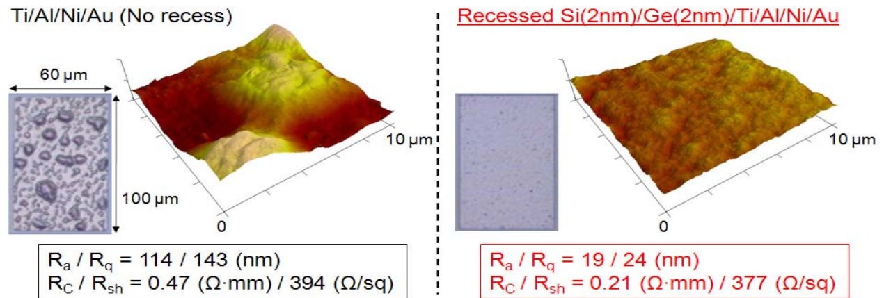
Figure 12. Comparison between conventional (left) and recessed Si(2nm)/Ge(2nm)/Ti/Al/Ni/Au ohmic contacts (right). Both of them were alloyed at 820 °C. 83% smoother surface roughness was observed for the new ohmic technology by AFM and microscopy images (inset).
