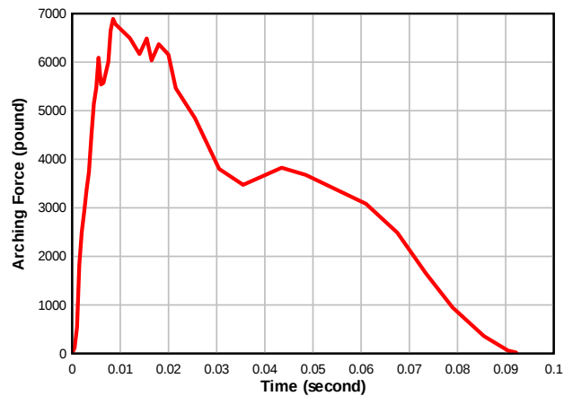
Figure 15. Arching Forces for Test 3.
