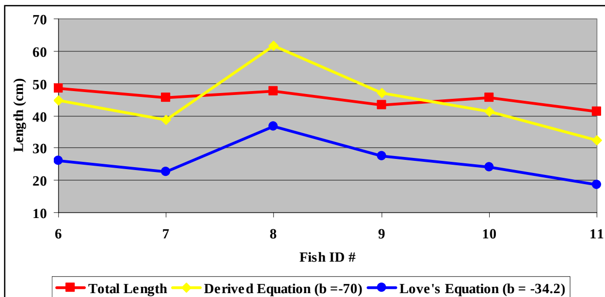
Figure 10. Comparison of measured and calculated total lengths at 200 kHz.
