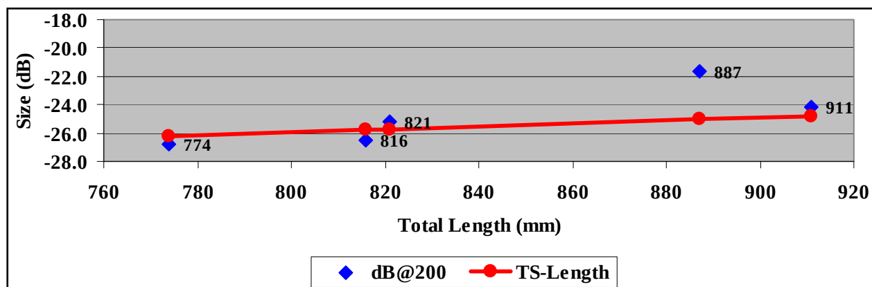
Figure 5. Measured TS in relation to calculated TS at 200 kHz.
