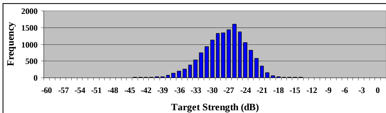
Figure 3. Target strength distribution for Sturgeon #2 at 200 kHz.
