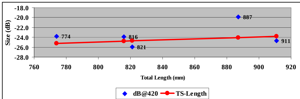
Figure 7. Measured TS in relation to calculated TS at 420 kHz.
