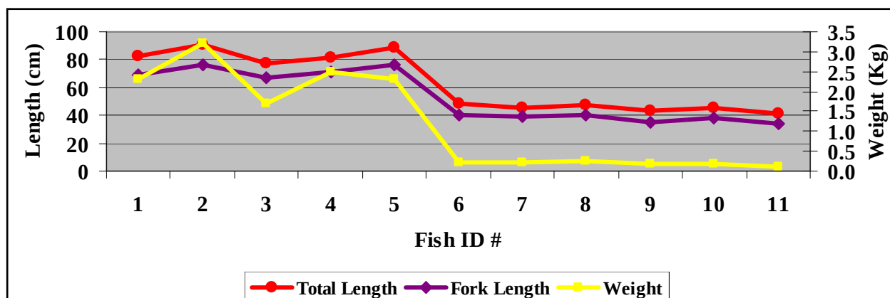
Figure 13. Comparison of total and fork length (cm) to weight (Kg)
