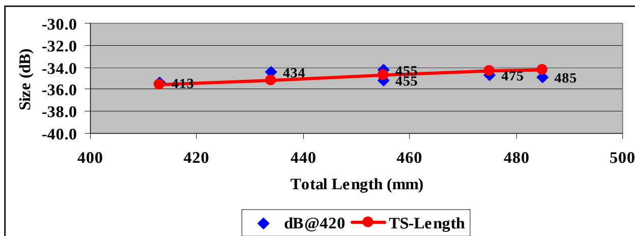
Figure 11. Measured TS in relation to calculated TS at 420 kHz.
