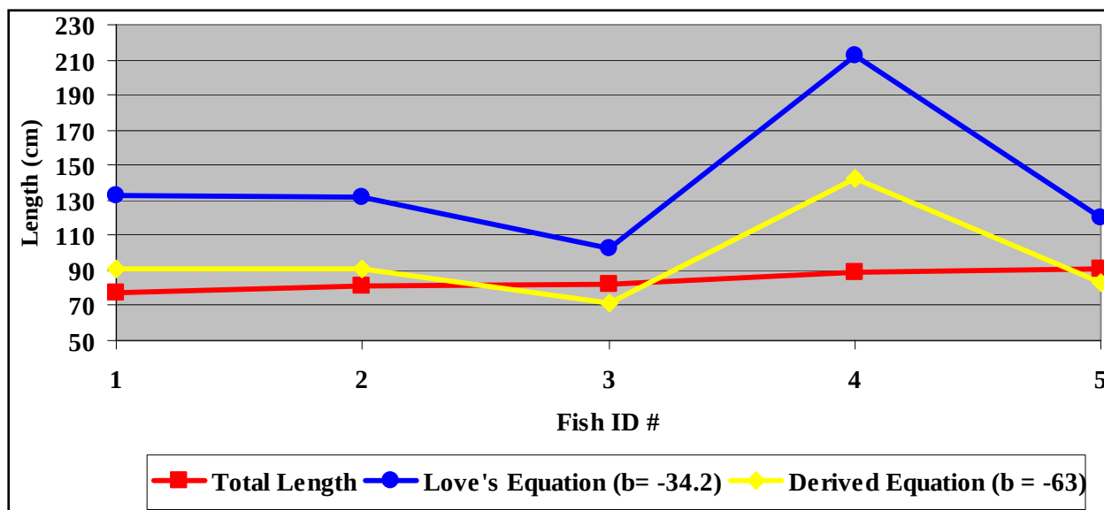
Figure 8. Comparison of measured and calculated total lengths at 420 kHz.
