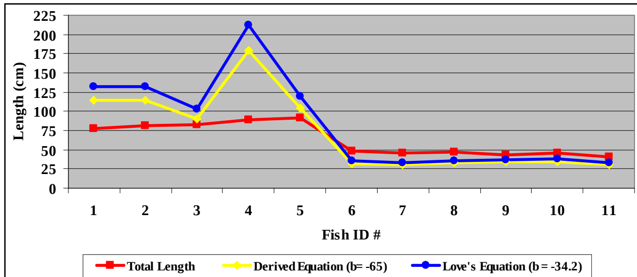
Figure 17. Measured versus calculated total length at 420 kHz.
