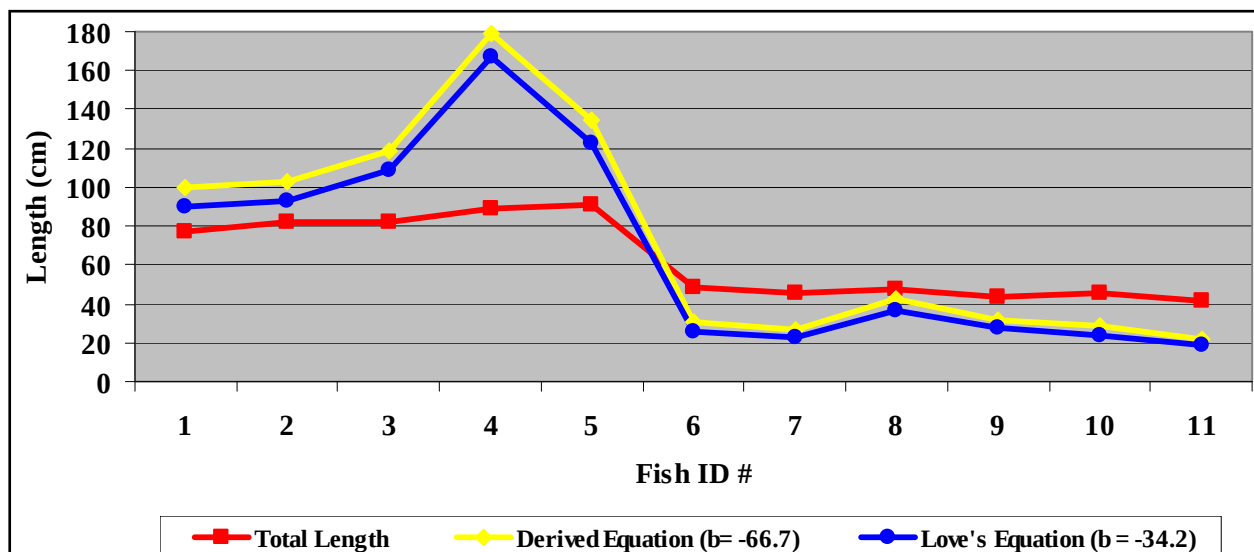
Figure 16. Measured versus calculated total length at 200 kHz.
