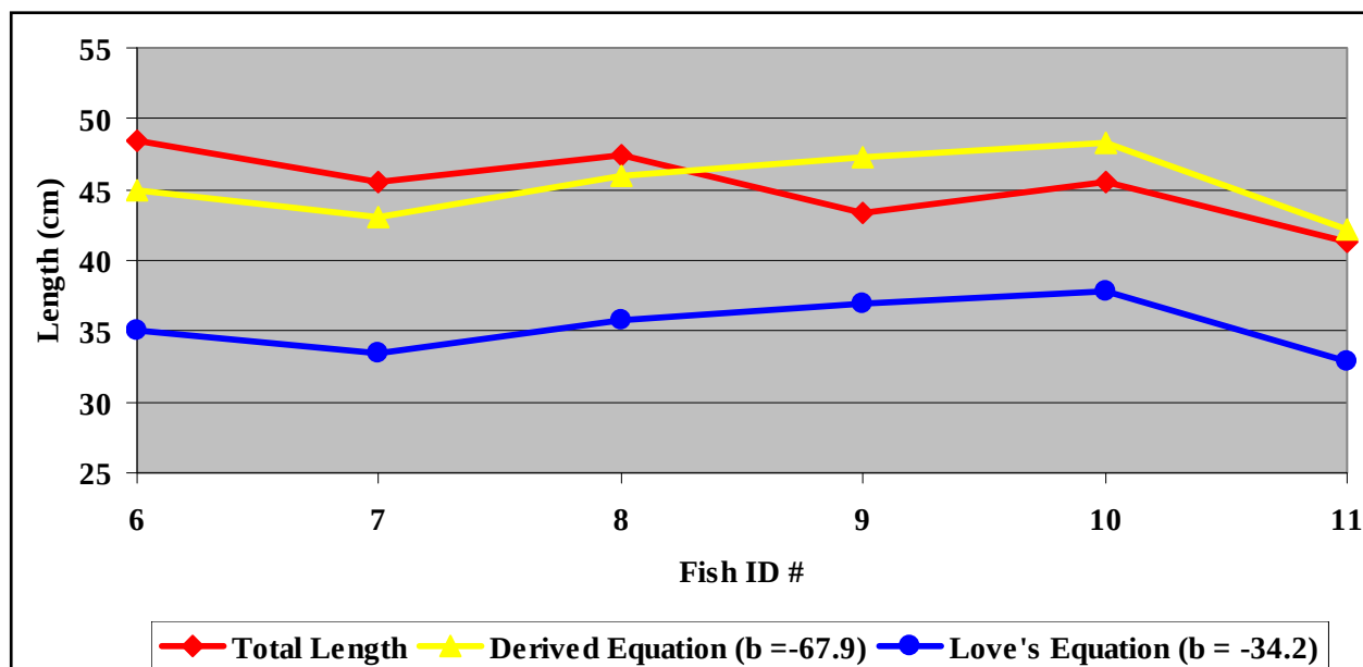
Figure 12. Comparison of measured and calculated total lengths at 420 kHz.
