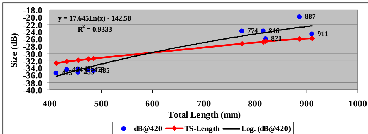
Figure 15. Relationship between measured total length and the natural log of calculated TS-length at 420 kHz.
