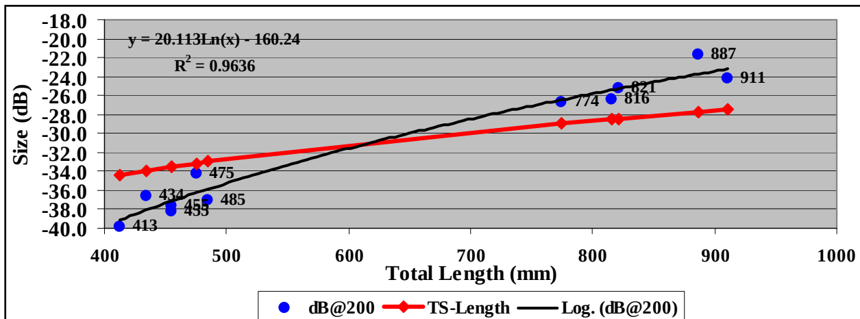
Figure 14. Relationship between measured total length and the natural log of calculated TS-length at 200 kHz.
