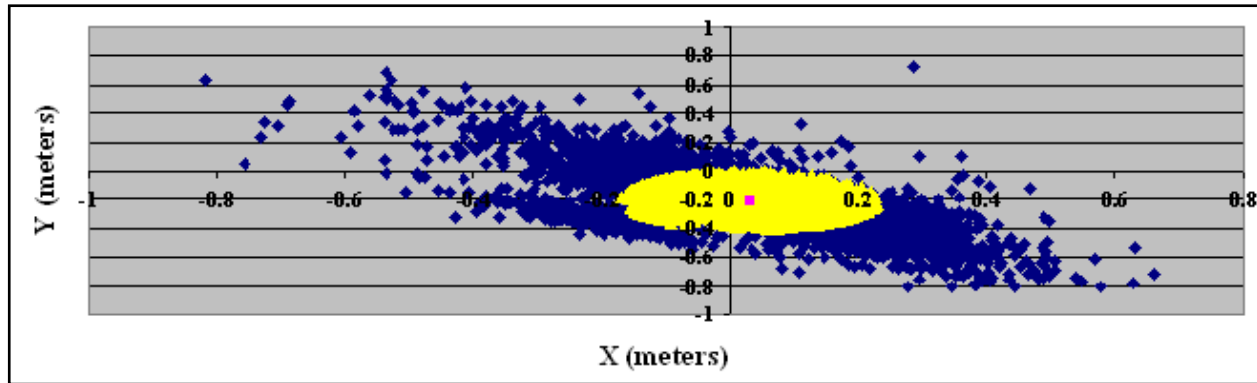
Figure 4. Distance (m) off-axis in the X and Y plane for acoustic returns of Sturgeon #5 at 420 kHz.
