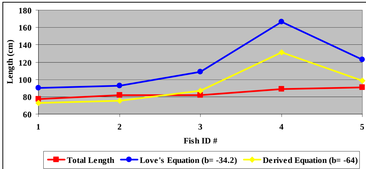
Figure 6. Comparison of measured and calculated total lengths at 200 kHz.
