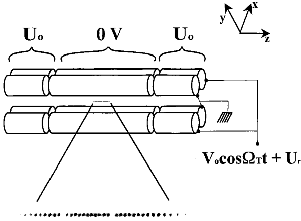
Fig. 1. The upper part of the figure shows a schematic diagram of the electrode configuration for a linear Paul-rf trap (rod spacing \approx 1\text{ mm} ). The lower part of the figure shows an image of a string of ^{199}\text{Hg}^+ ions, illuminated with 194\text{ nm} radiation, taken with a uv-sensitive, photon counting imaging tube [74]. The spacing between adjacent ions is approximately 10\text{ }\mu\text{m} . The “gaps” in the string are occupied by impurity ions, most likely other isotopes of \text{Hg}^+ , which do not fluoresce because the frequencies of their resonant transitions do not coincide with those of the 194\text{ nm } ^2\text{S}_{1/2} \rightarrow ^2\text{P}_{1/2} transition of ^{199}\text{Hg}^+ .
