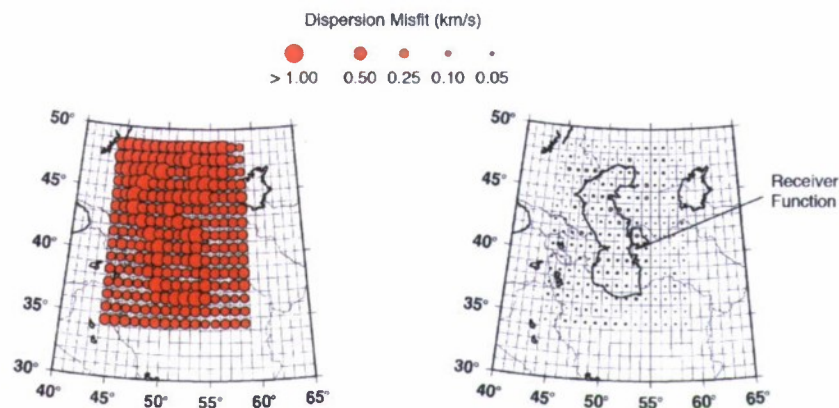
Figure 7. Initial (left) and final (right) dispersion misfit associated with the example subregion inversion of dispersion and a receiver function. The initial model consists of a simple “continental” model and a Caspian Sea model. The initial misfits are large, but the convergence is reasonable to mean misfit values near or below 0.05 km/s. The cell containing the isolated receiver function is labeled.
