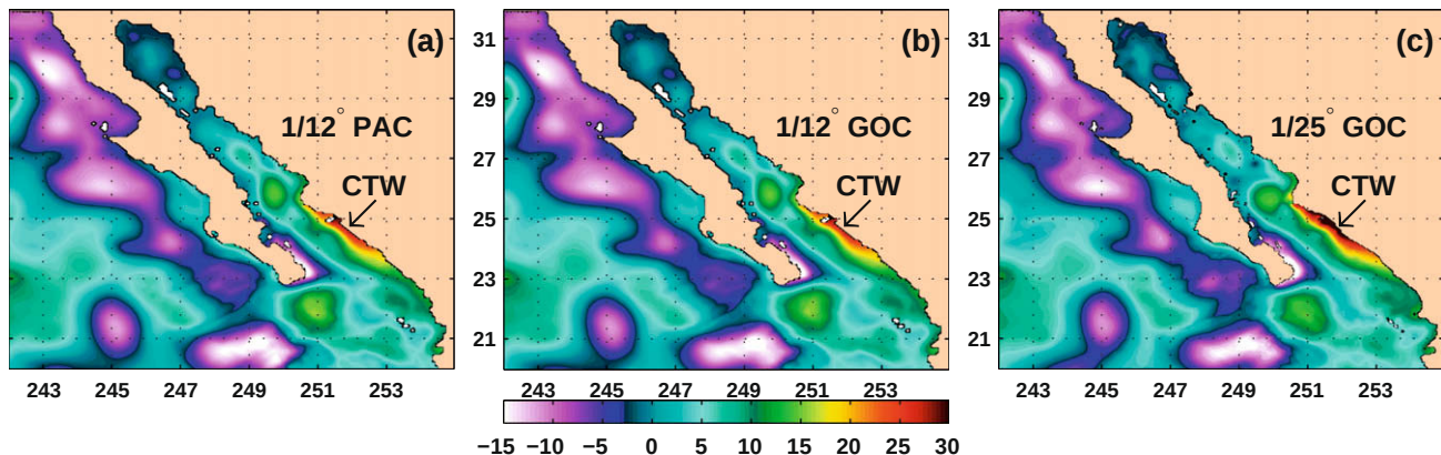
Fig. 4. Sea surface height snapshots (color contours in cm) for September 29, 2001 simulated with: (a) 1/12^\circ Pacific HYCOM, (b) 1/12^\circ GOC HYCOM, and (c) 1/25^\circ GOC HYCOM. The coastally trapped wave (CTW) was generated by Hurricane Juliette outside of the nested region and entered into the nested GOC models through the southern boundary.
