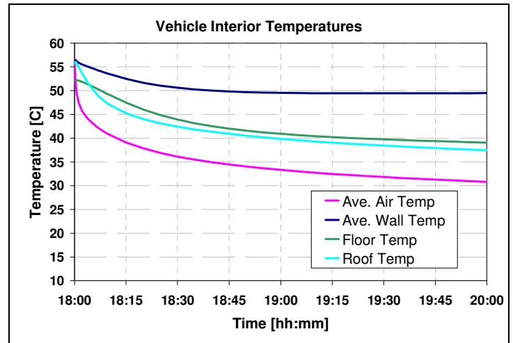
Figure 3: Vehicle interior average temperatures
