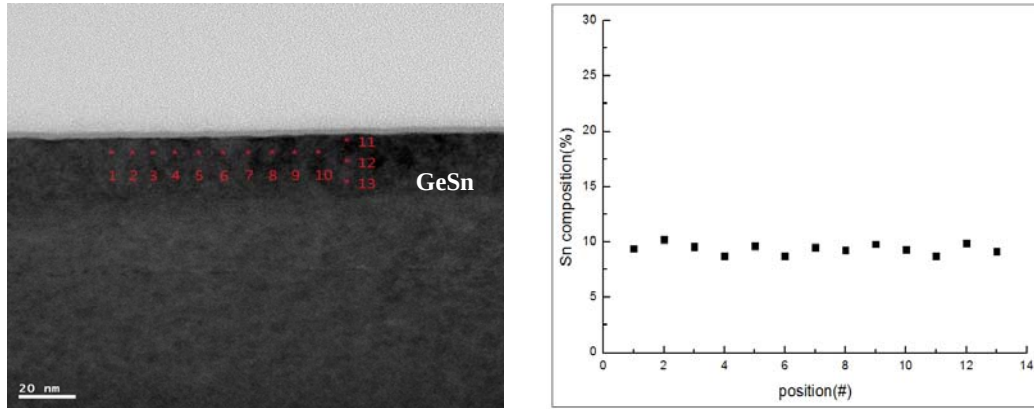
Fig. 2. (a) Left: STEM images of GeSn/Ge heterostructure with 10% Sn content. Dislocation associated with lattice misfit between GeSn and Ge is not observed in the GeSn layer showing the high quality of the growth. (b) Right: Sn content at various positions, as labeled in the left plot.
