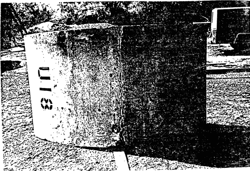
Figure 3. Typical Breakup for 0.09 Kg Charge Weight (Test 18)
