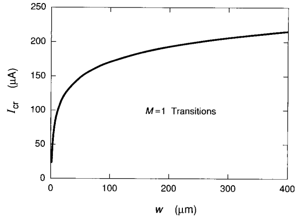
Fig. 12. The critical current I_{cr} versus sample width w . Refer to Sec. 5.4 for details of the calculation.
