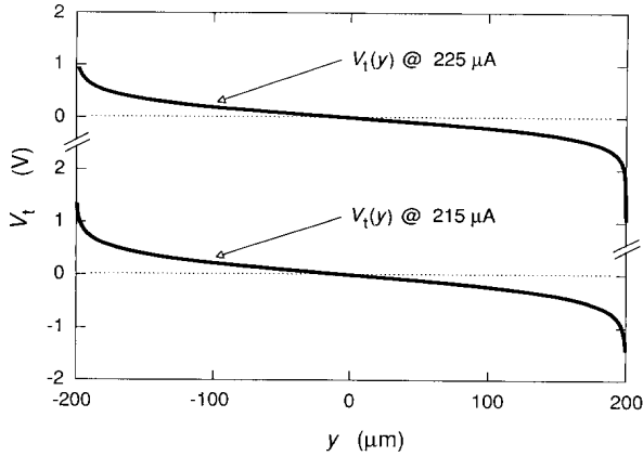
Fig. 6. V_t(y) plotted between y_{\max} and y_{\min} , using the parameters in Table 1 for I_{SD} = 215 \mu\text{A} and 225 \mu\text{A} . The values of y_{\max} and y_{\min} are 199.599 \mu\text{m} and -199.515 \mu\text{m} , and 199.901 \mu\text{m} and -198.044 \mu\text{m} for I_{SD} = 215 \mu\text{A} and 225 \mu\text{A} , respectively.
