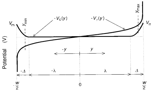
Fig. 4. The confining potential -V_c(y) and the charge-redistribution potential -V_r(y) across the sample for greatly exaggerated values of \Delta , \delta_{\max} = w/2 - y_{\max} , and \delta_{\min} = w/2 + y_{\min} .
