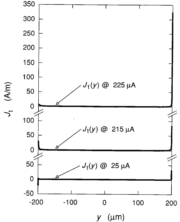
Fig. 9. Current density J_t(y) for I_{SD} = 25 \mu\text{A} , 215 \mu\text{A} , and 225 \mu\text{A} .
