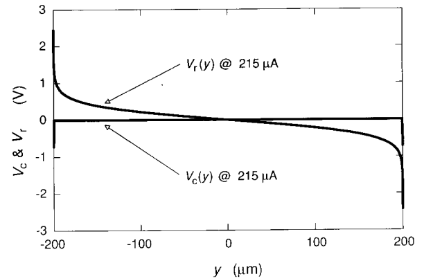
Fig. 5. V_c(y) and V_r(y) plotted between \pm 0.99999 w/2 for the parameters used in Table 1 at I_{SD} = 215 \mu\text{A} . The parameters common to all plots in Figs. 5–11 are i = 2 ( 12\,906.4 \Omega ), B = 12.3 \text{ T} , w = 400 \mu\text{m} , \kappa = 13.1 , \Delta = 0.5 \mu\text{m} , V_m = 0.75 \text{ V} , and G = 0.147 .
