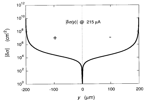
Fig. 11. Logarithmic plot of the charge-redistribution |\delta\sigma(y)| across the sample for I_{SD} = 215 \mu\text{A} , where \delta\sigma(y) is the deviation from the average number density n_s . The “-” region represents an excess of electrons, the “+” region a depletion of electrons.
