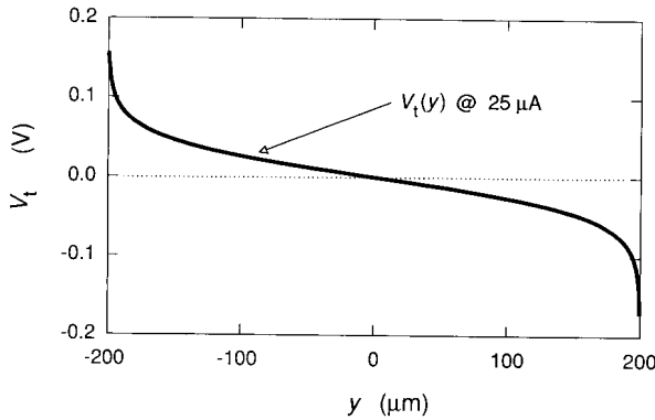
Fig. 7. V_t(y) at I_{SD} = 25 \mu\text{A} . This potential is in excellent agreement with the experimental measurements shown in Fig. 6 of Fontein et al. [8].
