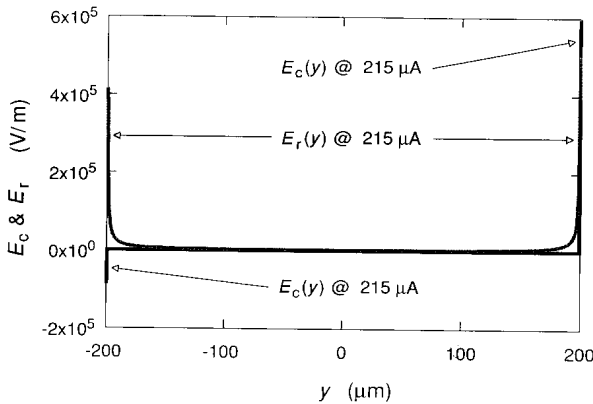
Fig. 8. Electric fields E_c(y) = -\nabla V_c(y) and E_r(y) = -\nabla V_r(y) for I_{SD} = 215 \mu\text{A} .
