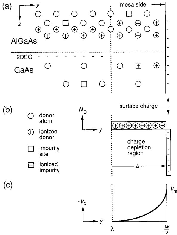
Fig. 2. (a) Schematic diagram of the GaAs/AlGaAs interface region near one side of the mesa. See Sec. 3.1 for further explanation. (b) The ionized donor charge-depletion density distribution N_D . (c) The confining potential V_c for negatively charged surface states.
