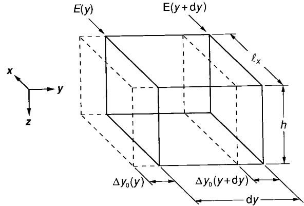
Fig. A-1. Geometry factors for the calculations in Appendix A.
