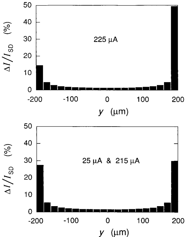
Fig. 10. Percentage of current flowing through 20 equal segments across the sample width for I_{SD} = 25 \mu\text{A} , 215 \mu\text{A} , and 225 \mu\text{A} .
