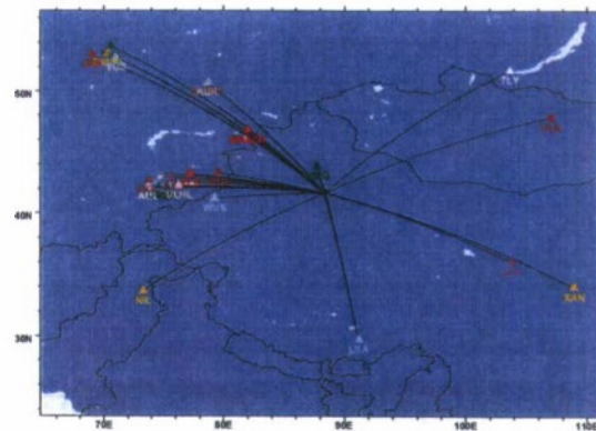
Figure 11. Locations of an earthquake pair during January 1999 at LNTS and regional stations.
