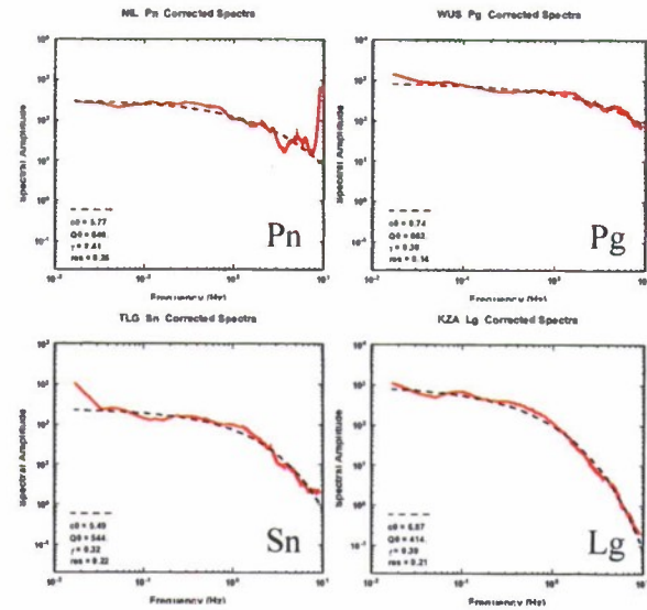
Figure 26. Examples of source-corrected spectra and Q model fits using a pair of LNTS earthquakes.
