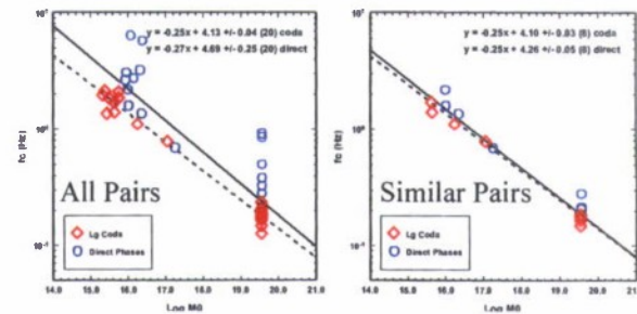
Figure 22. Estimates of source parameter for a cluster in Kazakhstan, using 10 events within 50 km of the master (left) and restricting the events to those with similar waveforms/mechanisms (right).
