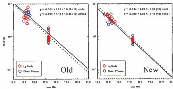
Figure 15. Source parameter estimates for 8 crustal pairs near LNTS using all regional data (left) and restricting the data by magnitude/distance (right).
