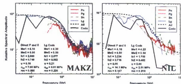
Figure 12. Relative spectra and source model fits at MAKZ (left) and NIL (right) for the LNTS pair.
