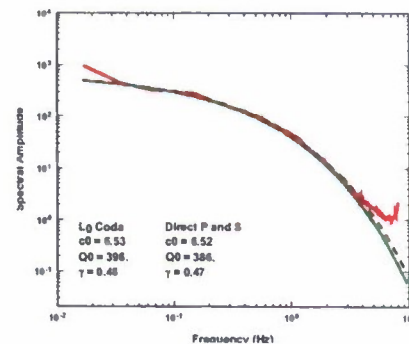
Figure 3. Source-corrected Lg spectra at BRVK for 100 events in the cluster (blue), the median (red), and Q model fits (black dashed and green) using source corrections from direct phases and coda, respectively.
