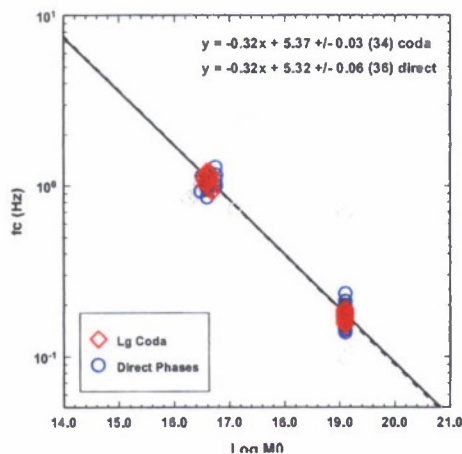
Figure 9. Single-station estimates of corner frequency versus log moment and scaling relations (linear fits) from direct phases and Lg coda. Gray markers correspond to stations with data quality problems.
