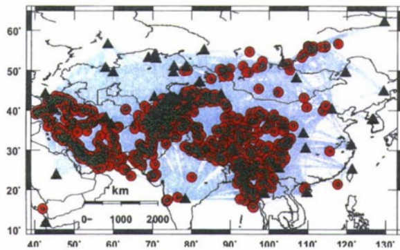
Figure 5. Map of earthquakes listed in the PDE from 1989 to 2009; red circles correspond to mb>5 events within 50 km of smaller events (green circles). Also shown are ray paths for which regional seismic data are available from IRIS stations (triangles).
