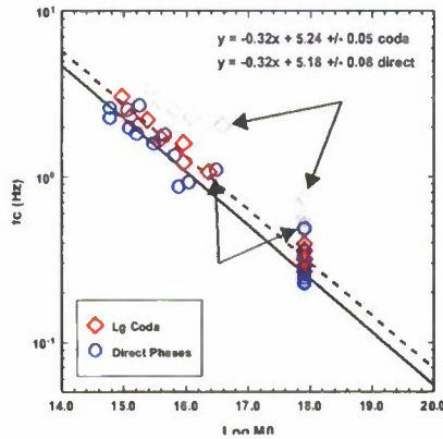
Figure 24. Estimates of corner frequency versus log moment and scaling relations from direct phases and Lg coda, using data from up to five common stations. Gray markers are outliers of the coda results.
