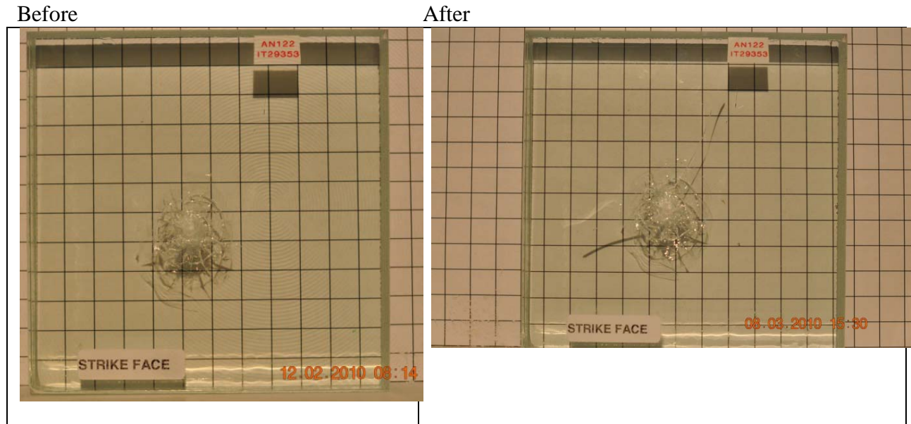
Note how much the cracks at 1:00 and 8:00 have extended as a result of thermal shocking.
