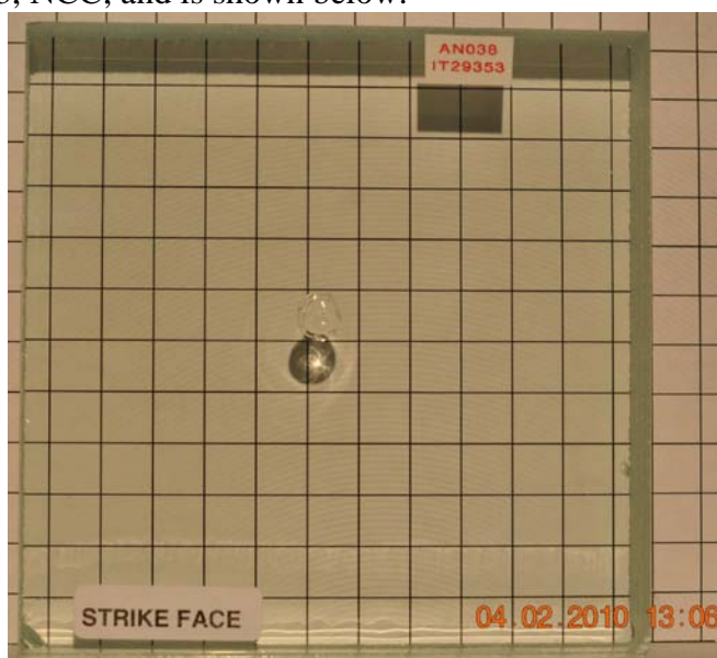
Photograph 2. Minor Damage at 129 f/s.
