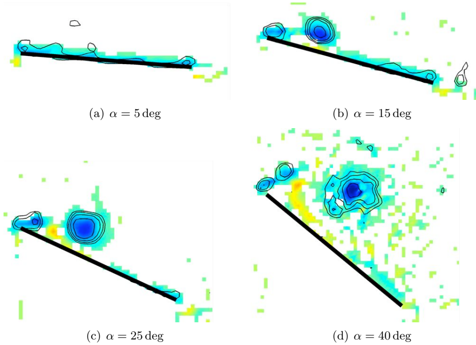
FIGURE 28. Vorticity field (at 3/4 span) at the lift minimum, x/c = 1.40 .
