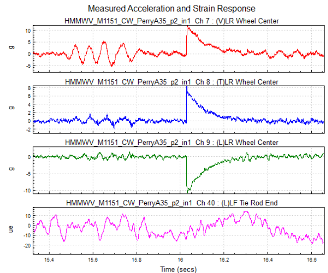
Figure 16: Input anomaly in experiment 8, test 2.
