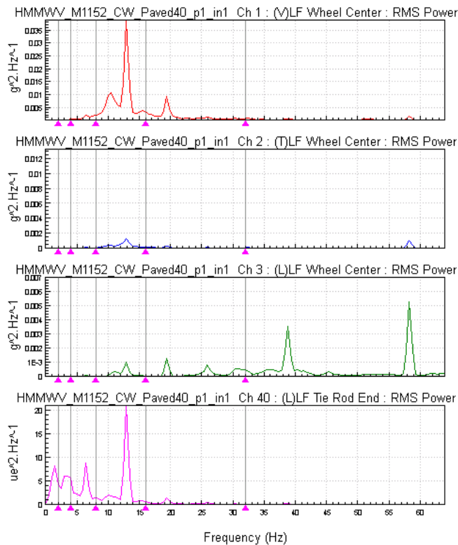
Figure 11: PSD of Input and Response Channels – Paved @ 40mph
