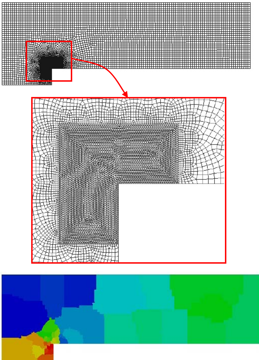
Figure 7. Mixed-type mesh and partition for MPI parallel processing.
