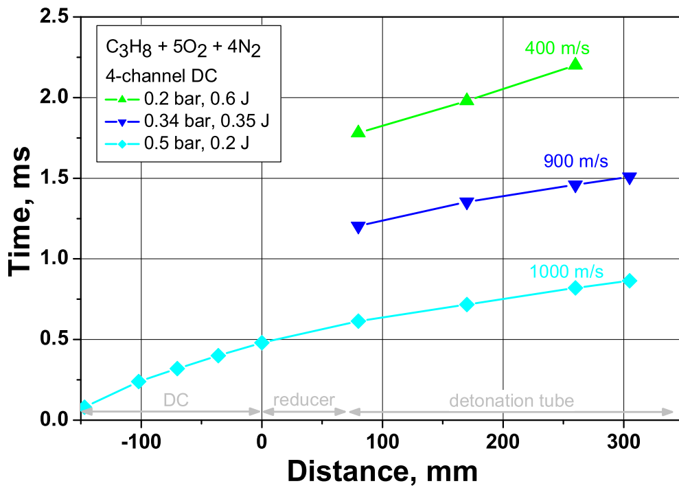
Fig. 3.25: X–t diagrams of DDT at initial pressures of 0.2–0.5 bar, streamer mode.
