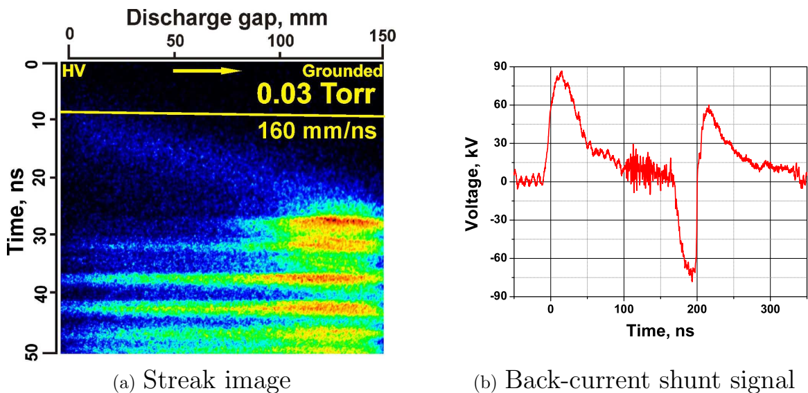
Fig. 2.8: Discharge development in the single-cell geometry. Air, 0.03 Torr, E/N = 10^6 Td, streamer velocity — 8 mm/ns.
