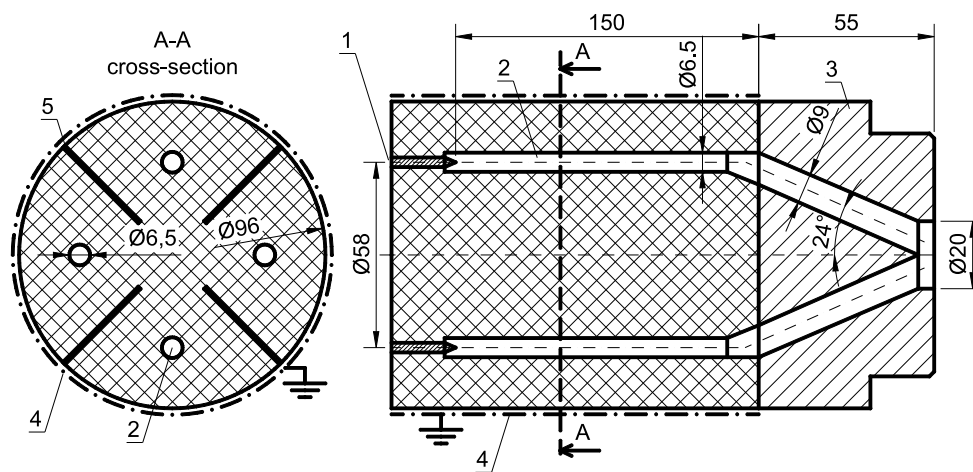
Fig. 3.1: Four-cell discharge chamber: the scheme. (1) — high-voltage electrode, (2) — discharge channel with a diameter of 6.5 mm, (3) — converging reducer, (4) — coaxial grounded shield, (5) — grounded plates.
