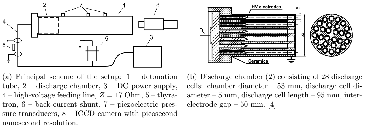
Fig. 1.4: The setup for detonation initiation with microsecond spark discharge.
