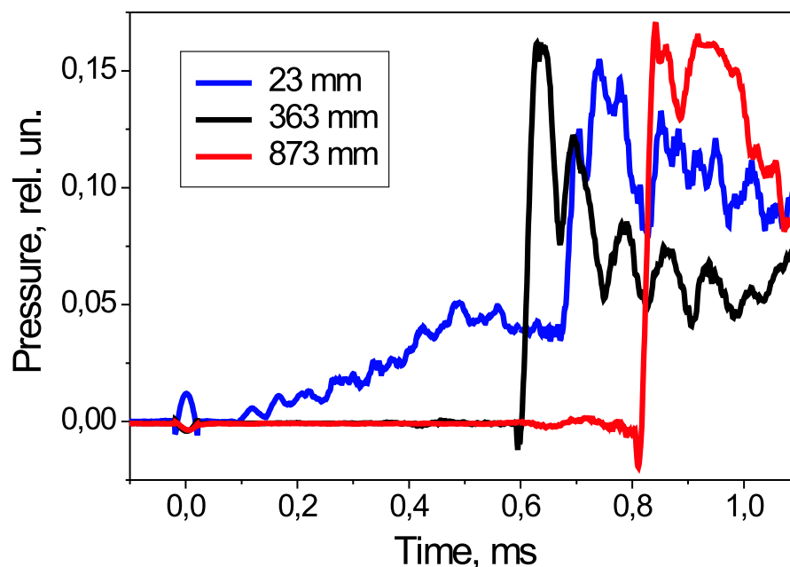
Fig. 1.5: A typical oscillogram of the pressure transducers signals. The distance from the discharge section is shown in the figure for every transducer. Initial mixture pressure 0.6 bar. Mixture: C_3H_8/C_4H_{10} + 5O_2 . Detonation, shock wave velocity 2350 m/s measured between transducers 2 and 3. C-J velocity for the given mixture \sim 2400 m/s.
