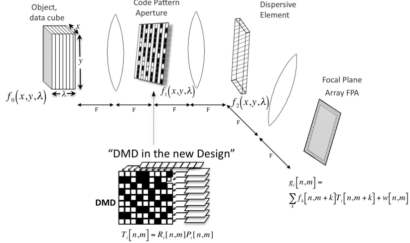
Figure 5: Representation of the CAASI parts. The fix code aperture in the traditional CASSI system is replaced by a spatial light modulator.
