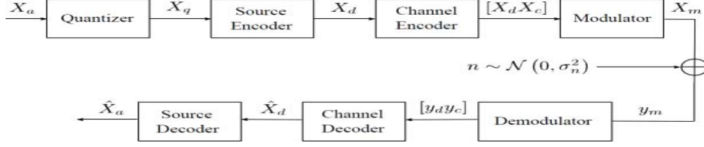
Figure 7: Block diagram of a Bit Interleaved Coded Modulation(BICM) system over AWGN channel.
