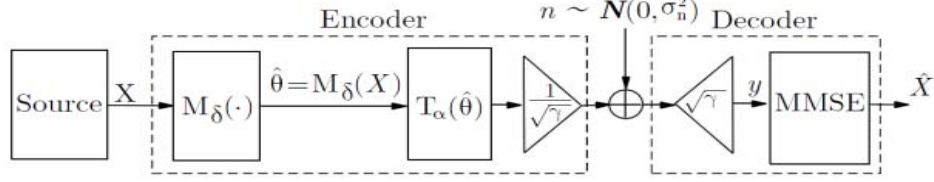
Figure 6: Block diagram of an N:1 bandwidth compression analog joint source-channel coded system.
