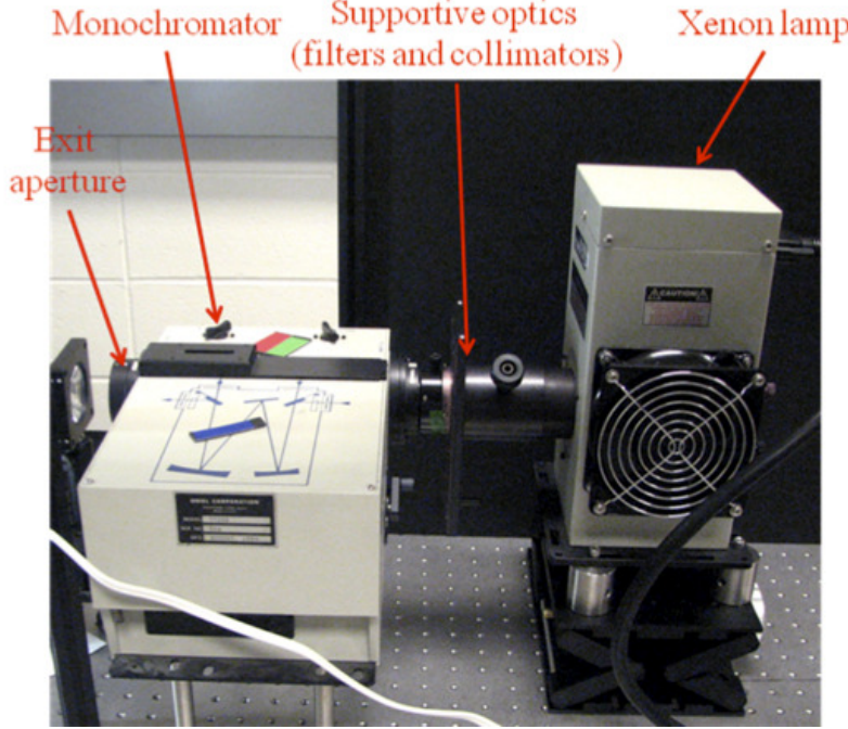
Figure 1: Monochromator setup. The output spectrum of the monochromator can be adjusted by rotating blazing-grating. The spectrum-range is 440-670nm (visible).
