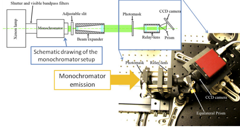
Figure 2: Experimental setup used to acquire the calibration cube using an equilateral prism with apex angle (apex angle: 60)
