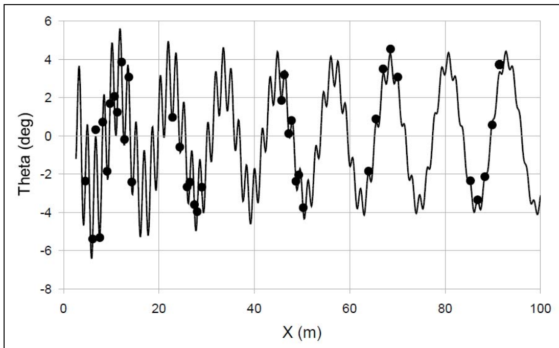
Figure A-1. Pitch angle vs. range for round 29271 (M855 at Mach 1.18).
