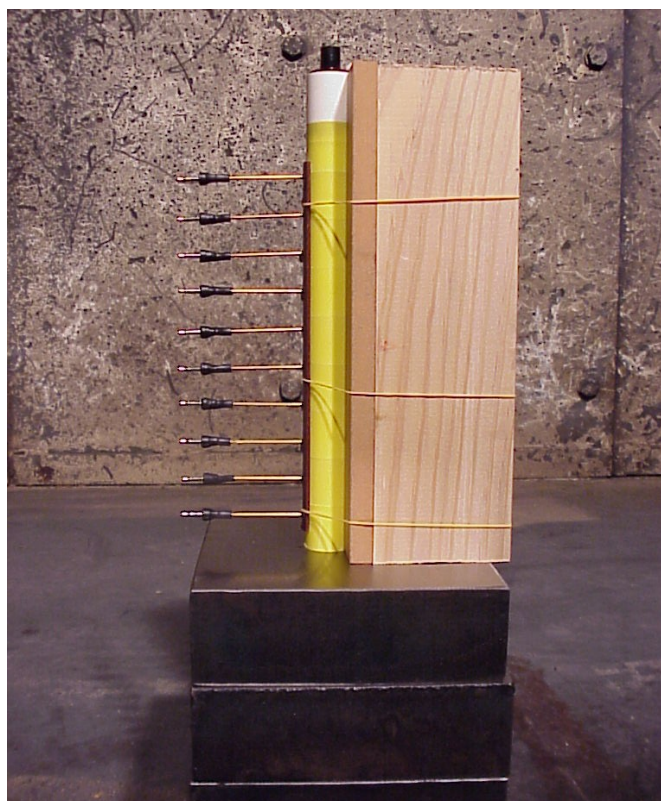
Figure 1: Velocity of detonation/detonation pressure experiment on FOX-7/EVA
