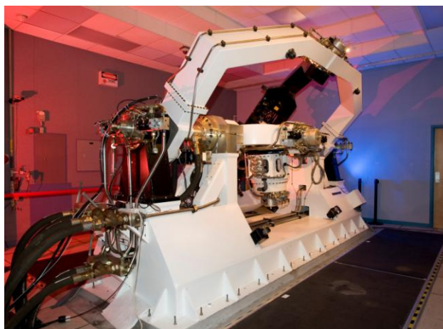
Figure 6. Carco 5-axis FMS & controller.
