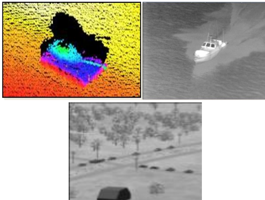
Figure 18. Ground and maritime RTC output in various wavebands.
