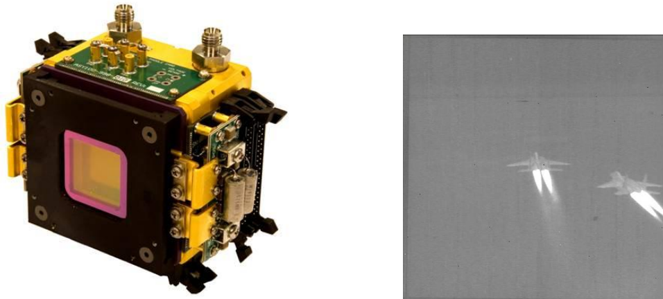
Figure 12. OASIS 512 x 512 IRSP (left), raw imagery captured with IR camera (right).
