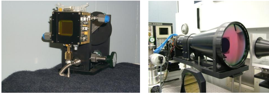
Figure 11. MSSP infrared projector (left), collimator optics (right).
