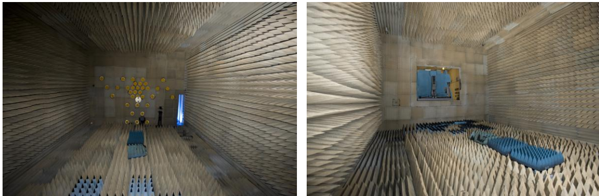
Figure 21. RF anechoic chamber.
