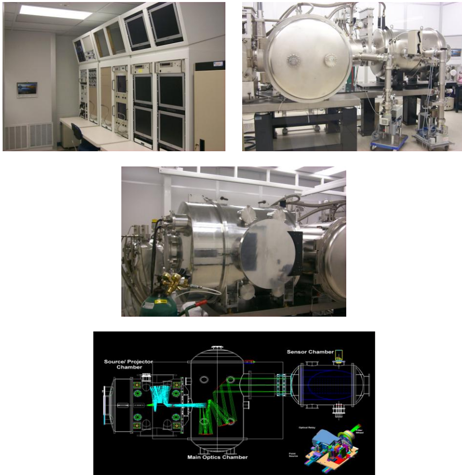
Figure 20. Cryogenic chamber.
