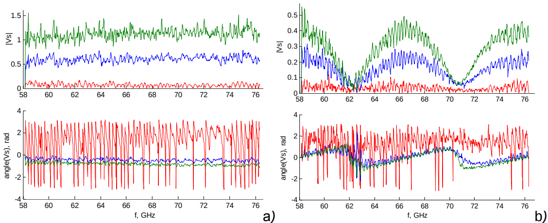
Fig. 13. Reflection coefficients from metal screen (a) and dielectric plane (b), moving over the antenna: red – screen on the edge of aperture projection, blue – screed half-shields the aperture projection, green – screen completely shields the aperture projection.
