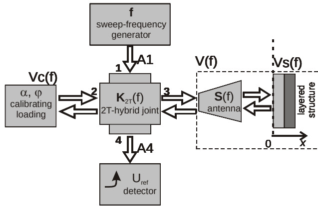
Fig. 8. Schematic model of test bench: f – generator of oscillating frequency; U_{ref} – detector of signal of reflected wave; V_c – CRF of calibrated load; K_{2T} – dispersion matrix of the double T-bridge; V(f) – CRF of load under measurement; S(f) – aerial; V_s(f) – CRF of flat-layered environment in free space
