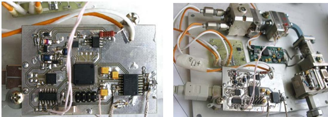
Fig. 6. Block of control and digital processing on the model of the NDT device.
