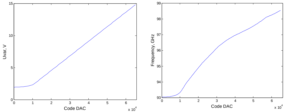
Fig. 5. Calibration of the device by frequency, dependence of voltage on varactor (a) and frequency (b) on the DAT code.
