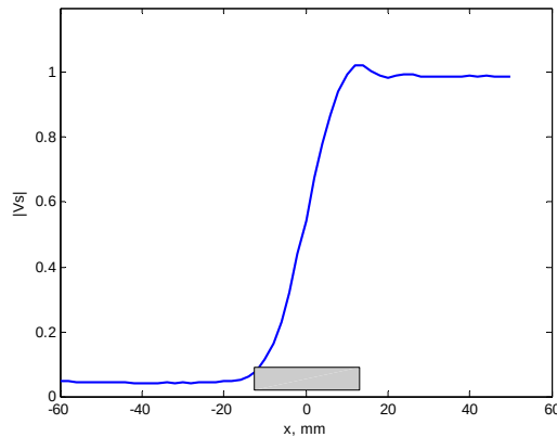
Fig. 14. Dependence of RC module on the position of screed related to the axis of antenna aperture.
