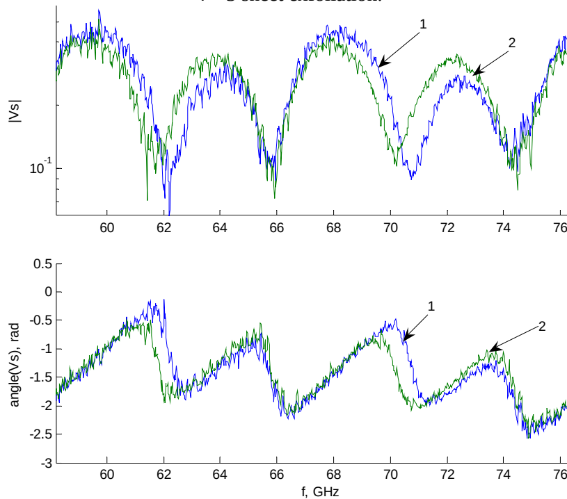
Fig. 5. Modeling of exfoliation in plate. Two plexiglass plates 10,5 mm, 1 – exfoliation of 3-sheet thickness with air; 2 – exfoliation with 2 sheets of paper.
