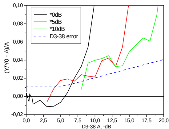
Fig. 7. Relative error of measured extinction coefficient.
