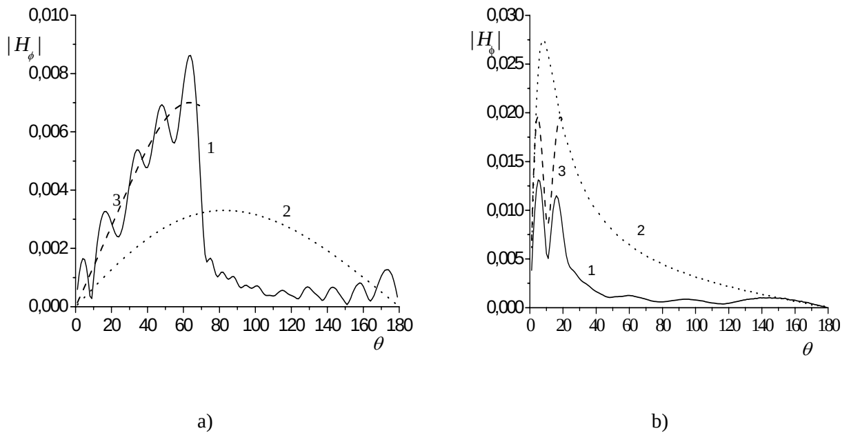
Fig. 4. Distribution of H_\phi – field components in vicinity of conical horn on a sphere of radius kr : 1 – whole field, 2 – primary field, 3 – field in semi-infinite come (a) kc_1 = 24 ; kl = 1,5 ; \gamma_1 = 70^\circ ; kr = 24,2 ; b) kc_1 = 12 ; kl = 10,5 ; \gamma_1 = 20^\circ ; kr = 12,2 .
