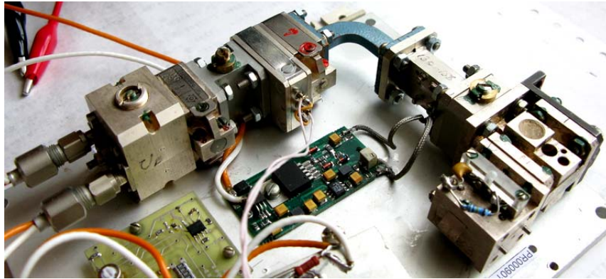
Fig. 15. Model of the unit for generation of 3-mm range.
