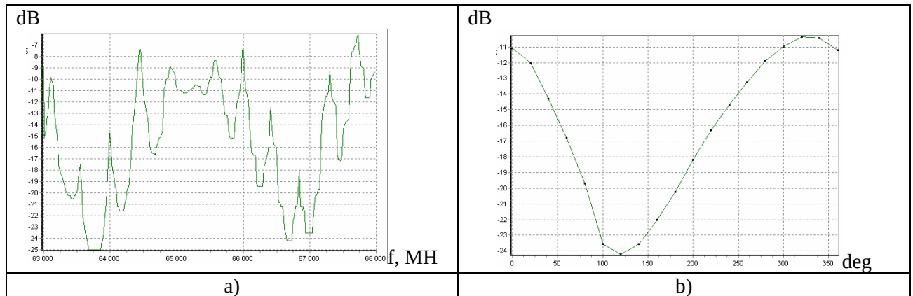
Fig. 9. Frequency and phase dependences of the disbalancing signal of the bridge scheme.
