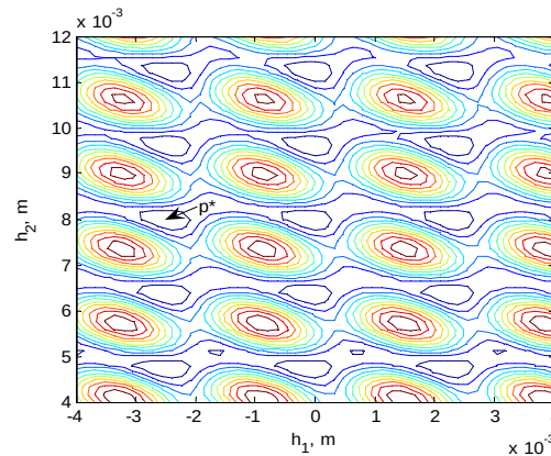
Fig. 9. Objective function of the IP for determination of location and thickness of the plate F(h_1, h_2) , p^* = (-0.00249; 0.00819) .
