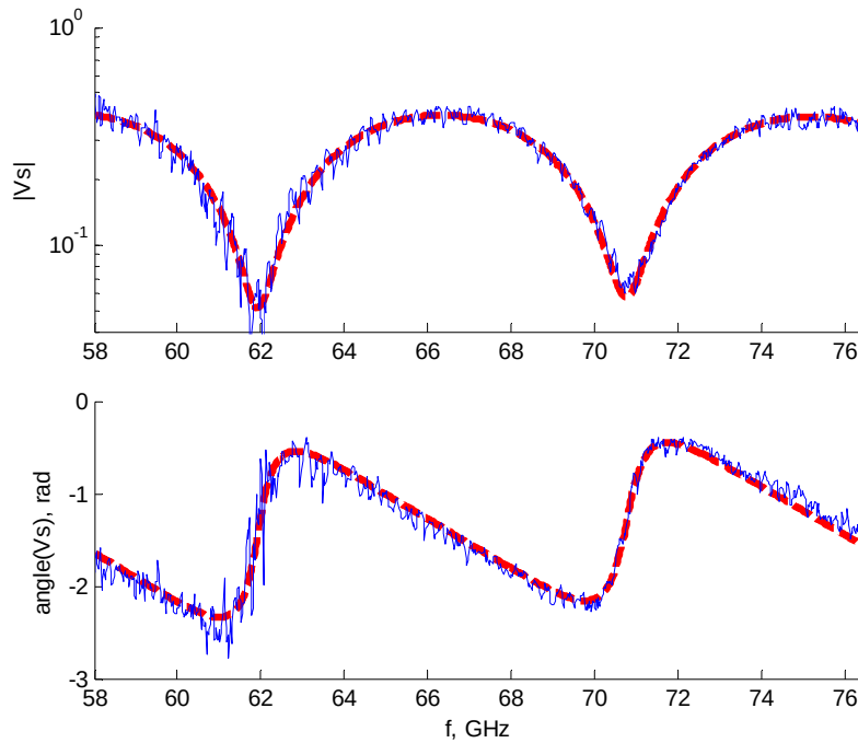
Fig. 3. Evaluation of the plexiglass plate parameters: h_1 = -0.358 mm, h_2 = 10.561 mm, \varepsilon_2 = 2.574 , tg \delta_2 = 6.31 \times 10^{-3} .
