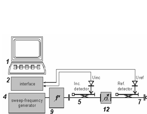
Fig. 6. Scheme of passing junction of attenuator: 12 – polarization attenuator
