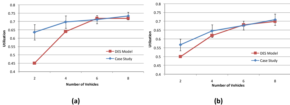
Figure 4.18 Mean utilizations from MUV-DES model and historical data set for a) NDS and b) FDS conditions
