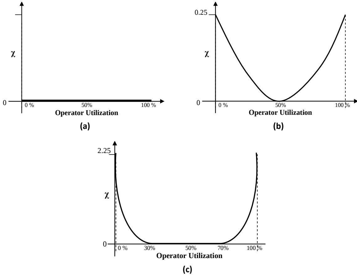
Figure 4.19 Situation Awareness Curve Variations
