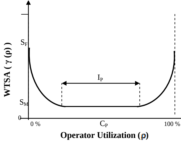
Figure 3.4 \gamma curve relating WTSA to \rho
