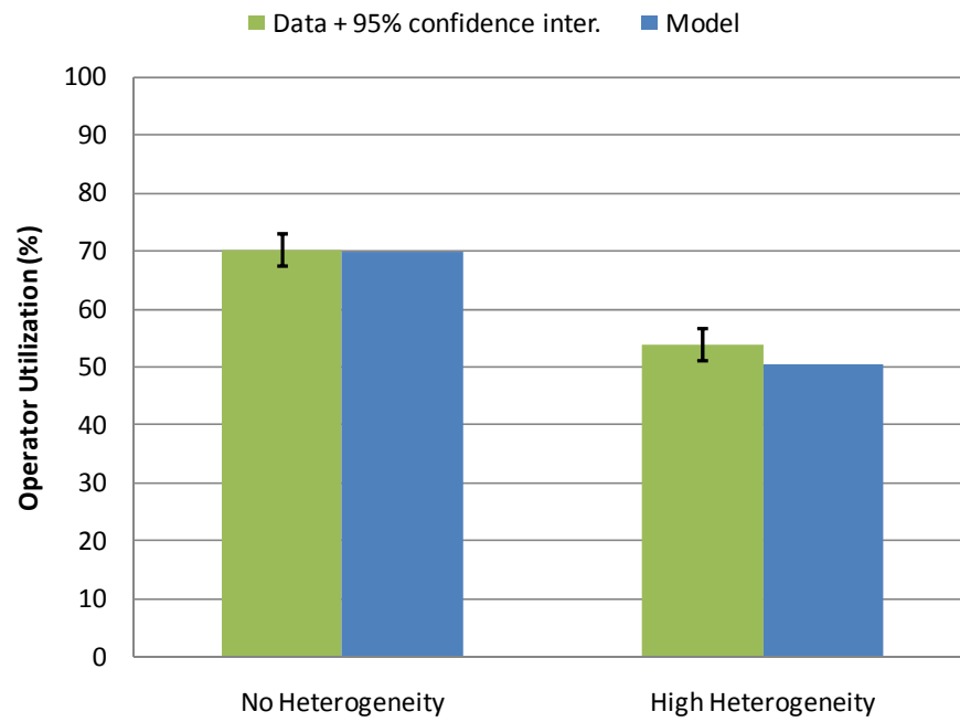
Figure 4.10 Results for operator utilization compared with model predictions
