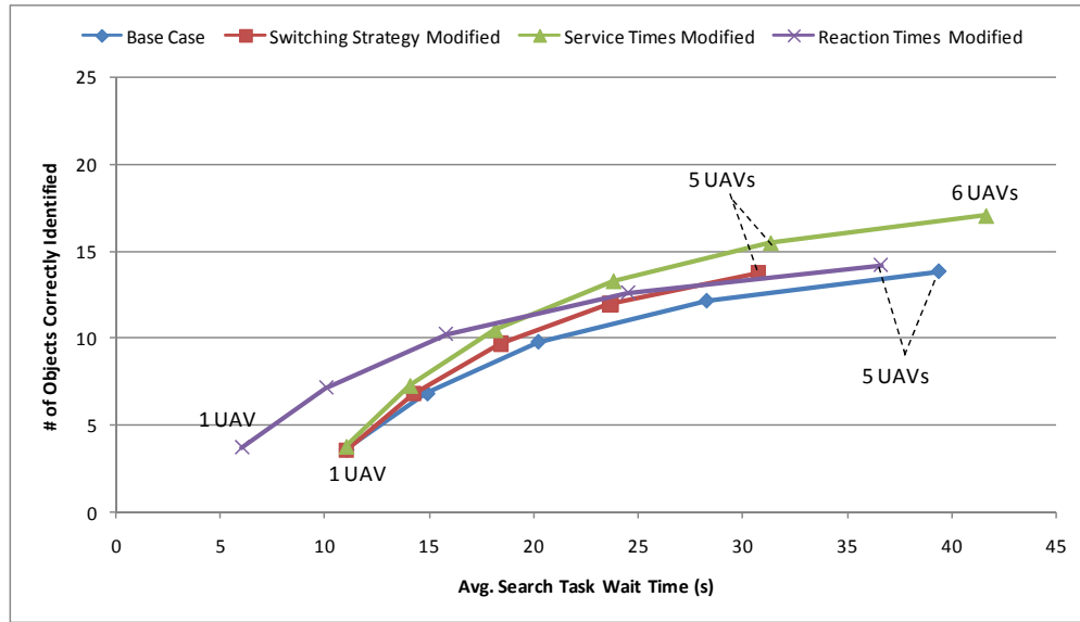
Figure 5.4 Tradeoff curve shift for independent variation of the switching strategy, interaction times, and penalties due to loss of SA
