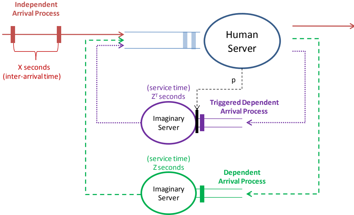
Figure 3.3 Three different arrival processes arriving to the MUV-DES server
