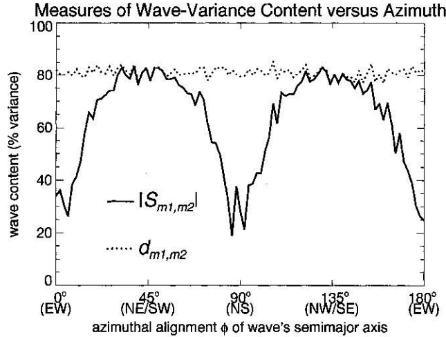
Figure 1. Comparison of the cross coherence |S_{m_1,m_2}| (= |\int_{m_1}^{m_2} \tilde{S}(m) dm|) and degree of polarization d_{m_1,m_2} , as computed from synthesized data. The synthesized vertical profiles contained an elliptically polarized wave ( |f/\omega| = 0.1 , where \omega is intrinsic frequency and f is inertial frequency) with a total horizontal-velocity variance of 25.25 \text{ m}^2 \text{ s}^{-2} and a vertical wavelength of 4 km. The semimajor axis of this coherent wave was aligned at an azimuth angle \phi and then sampled over a total height range of 40 km, and at a vertical resolution is 1 km to give two profiles of zonal and meridional velocities. Uncorrelated Gaussian noise with a variance of 10 \text{ m}^2 \text{ s}^{-2} was added to both the zonal and the meridional profiles. One hundred independent pairs of zonal and meridional velocity profiles were analyzed spectrally within a wavenumber band between m_1 = 2\pi (5 \text{ km})^{-1} and m_2 = 2\pi (3 \text{ km})^{-1} .
