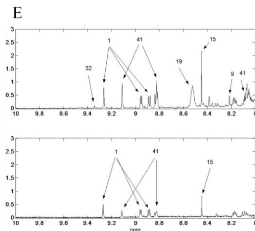
Figure 3: Representative annotated NMR traces (A – E) of predose (top pannel) and 24 hours D-serine post-dose (bottom pannel) rat urine.
