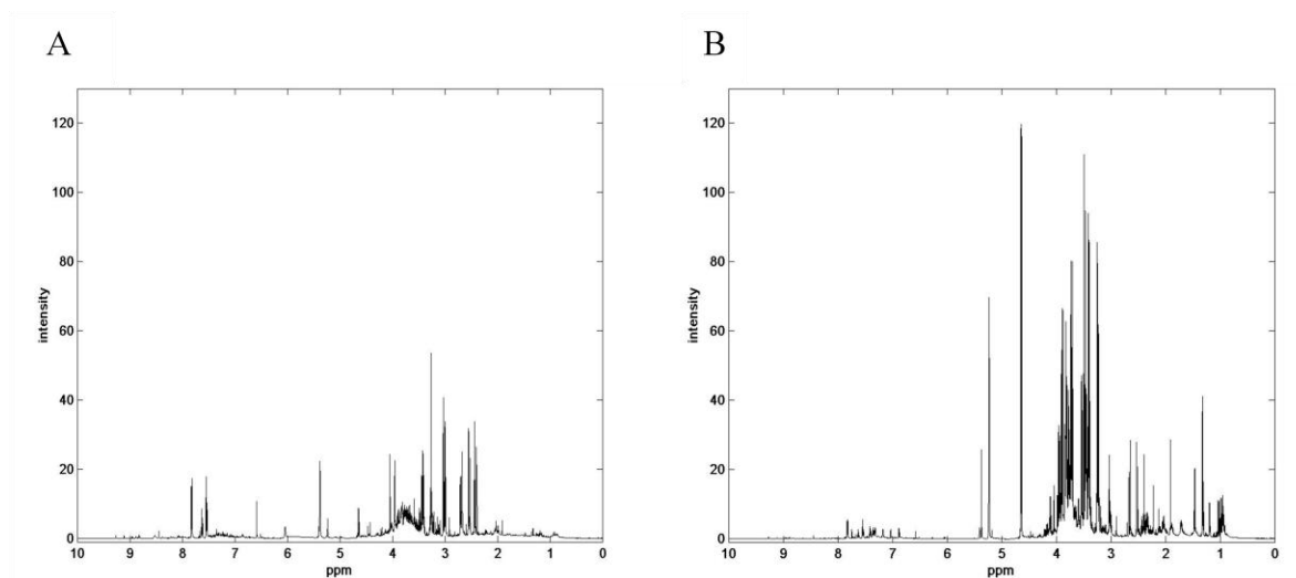
Figure 1: Representative 600 MHz ^1\text{H} NMR dosed rat urine spectra
