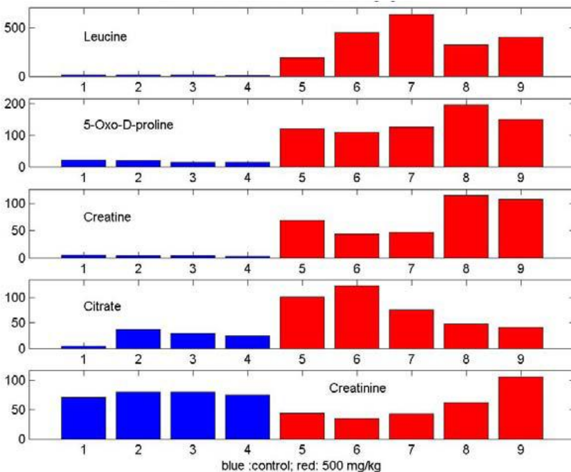
Figure 7: LC/MS normalized ion intensities across urine samples for tentatively identified metabolites: Leucine, -Oxo-D-Proline, Creatine, Citrate, and Creatinine
