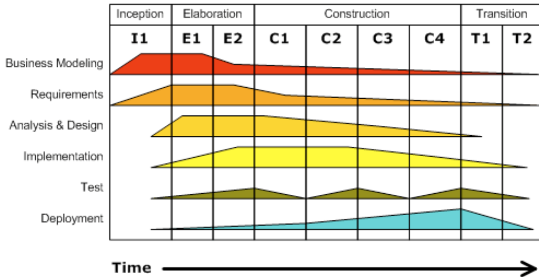
Figure 2. Unified Process (From Dutchguilder, 2007)
