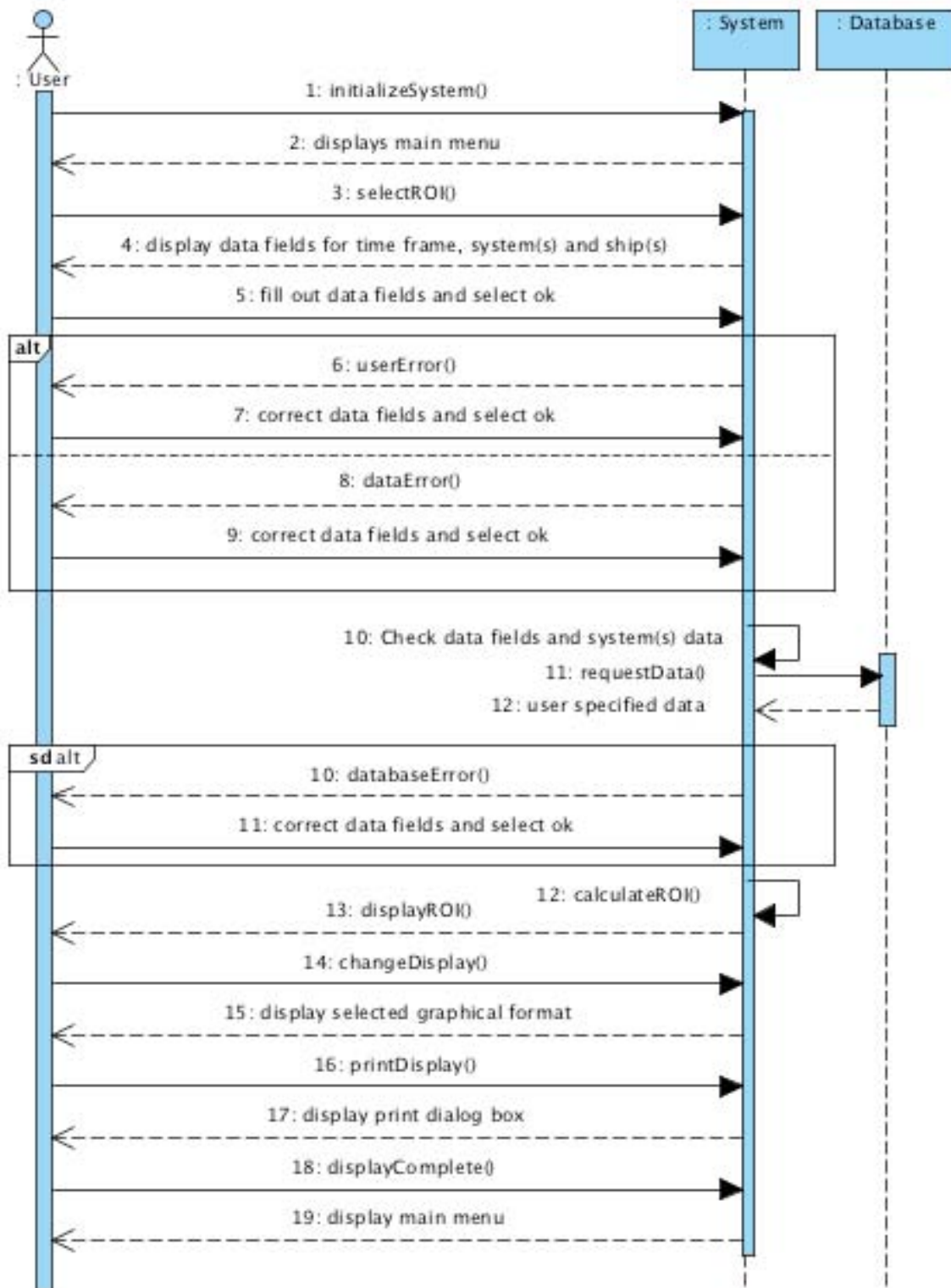
Figure 12. System Sequence Diagram for UC-1
