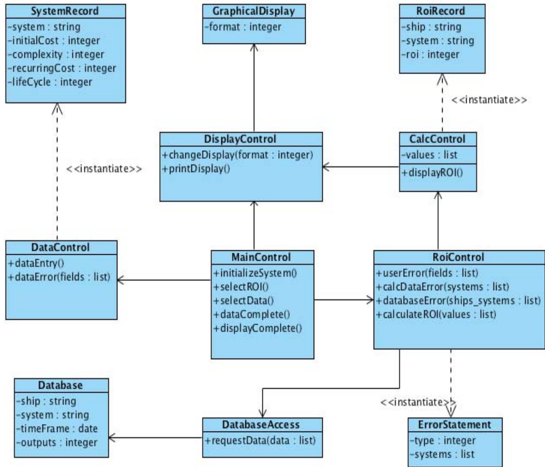
Figure 16. System Design Class Diagram
