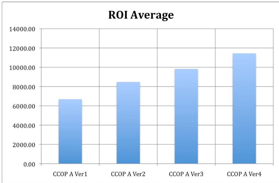
Figure 10. Graphical Display 2 Tab of Solution Prototype
