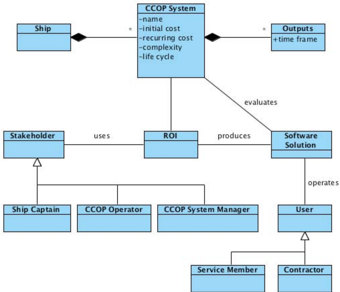
Figure 14. Domain Model for the System
