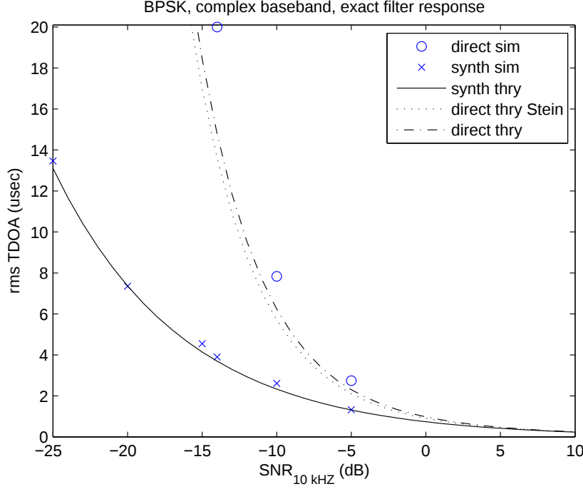
Figure 4: rms TDOA accuracy for a BPSK signal.
