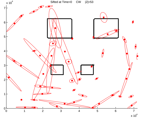
Figure 6: Predetection fusion on the first scan of data.
