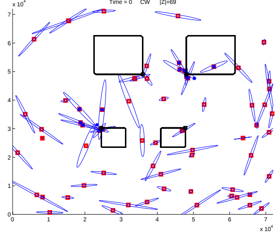
Figure 5: Winnowing on the first scan of data.
